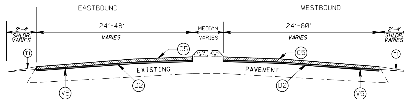
TYPICAL SECTION NO. 49
