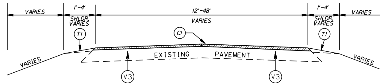
TYPICAL SECTION NO. 47
