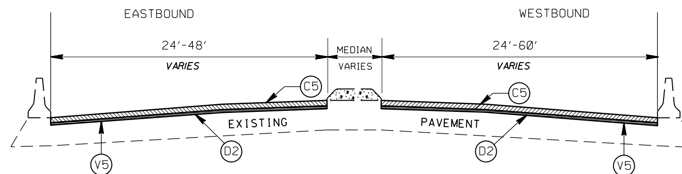
TYPICAL SECTION NO. 50
