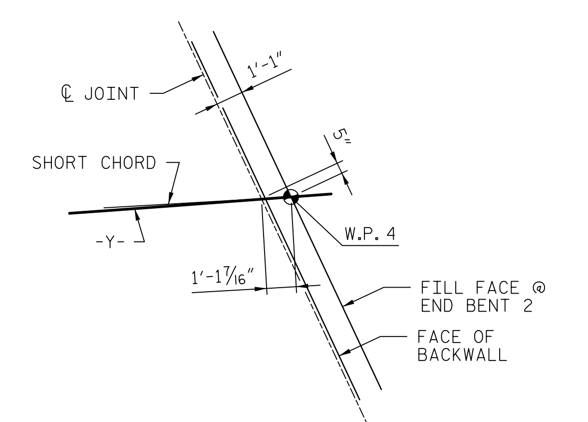
DETAIL "D"
