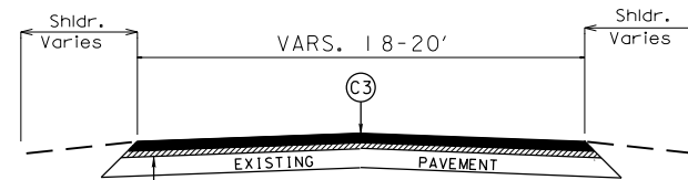
TYPICAL SECTION NO. 17
