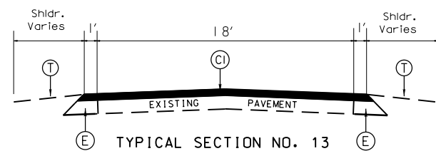
TYPICAL SECTION NO. 13
