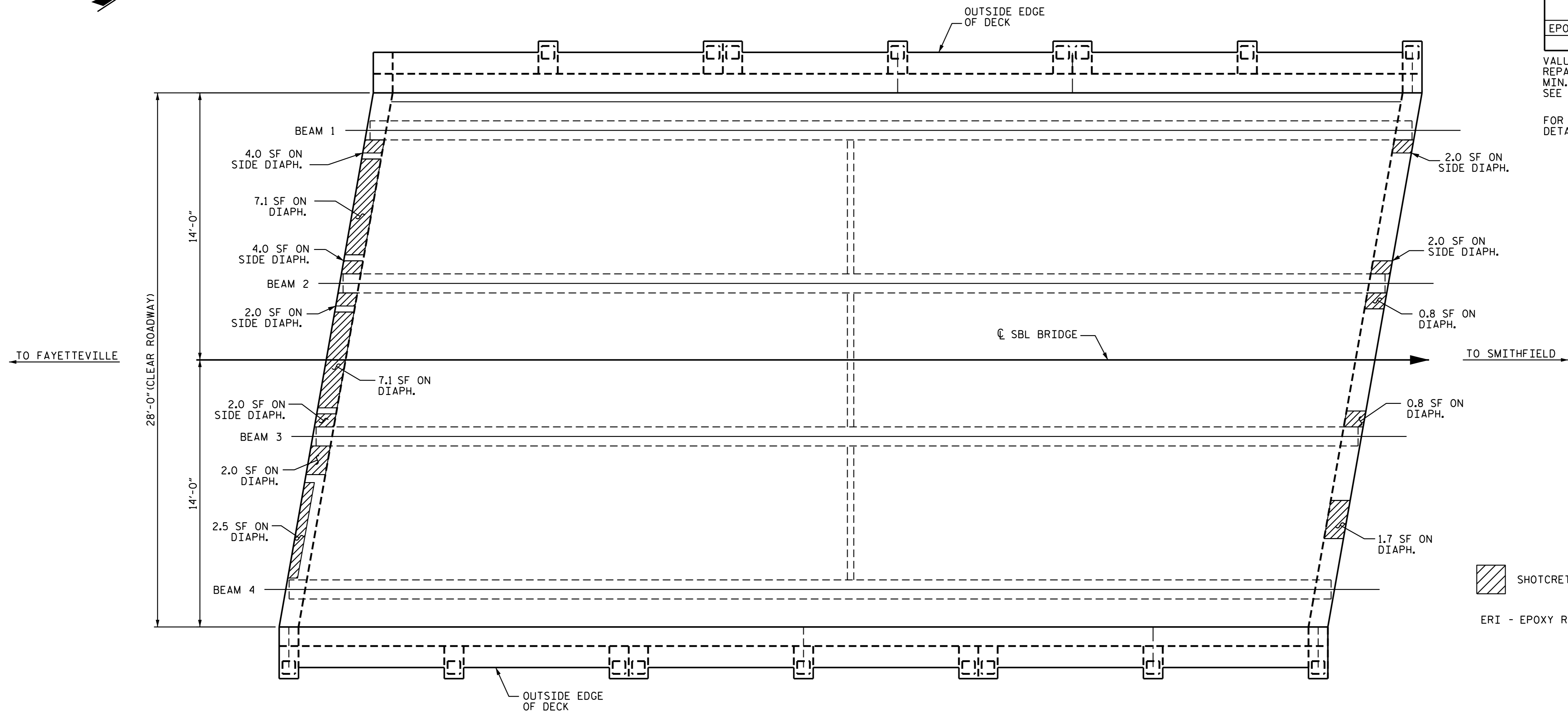
PLAN OF SPAN C UNDERSIDE
