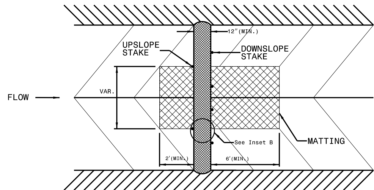
TOP VIEW
