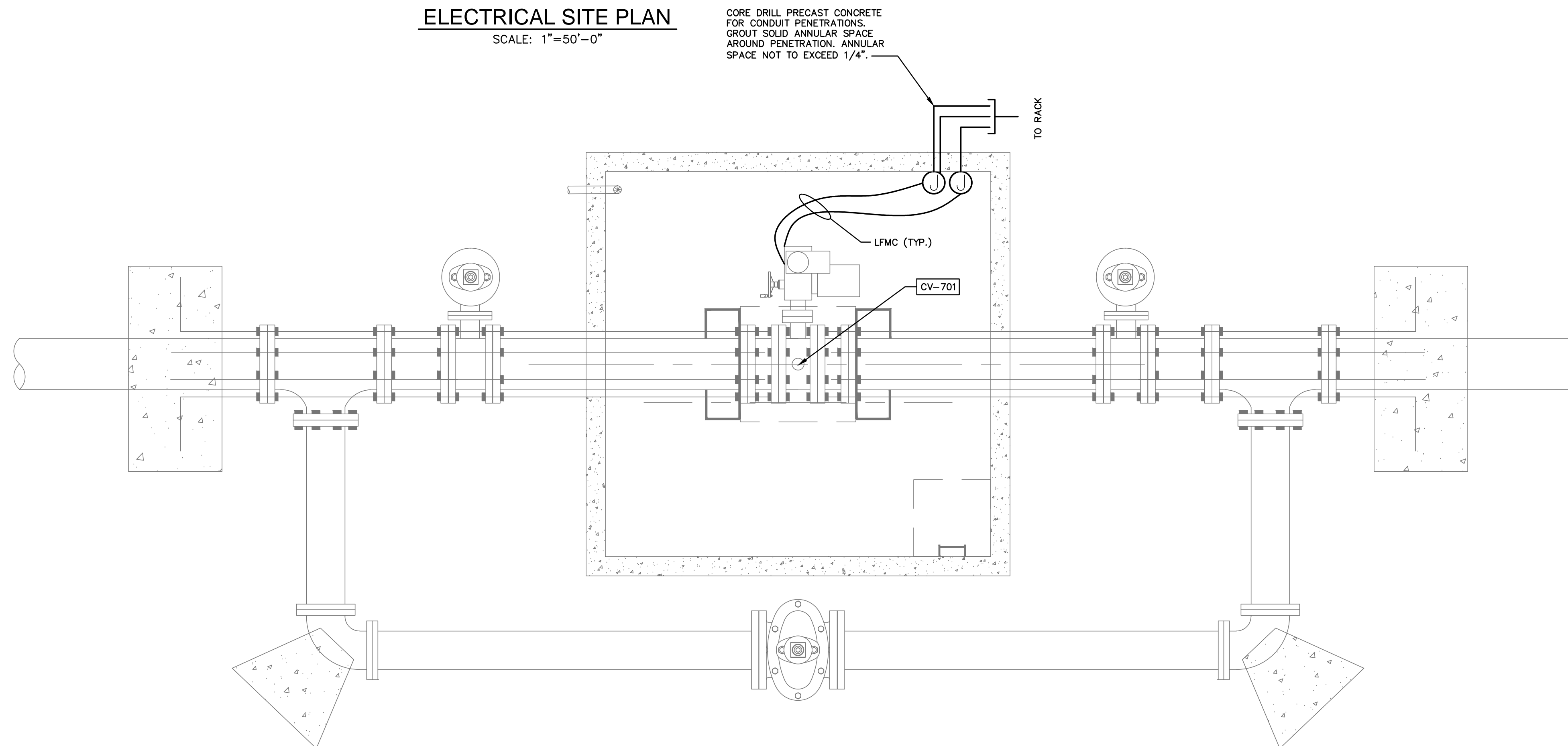
CONTROL VALVE VAULT ELECTRICAL PLAN NOT TO SCALE
