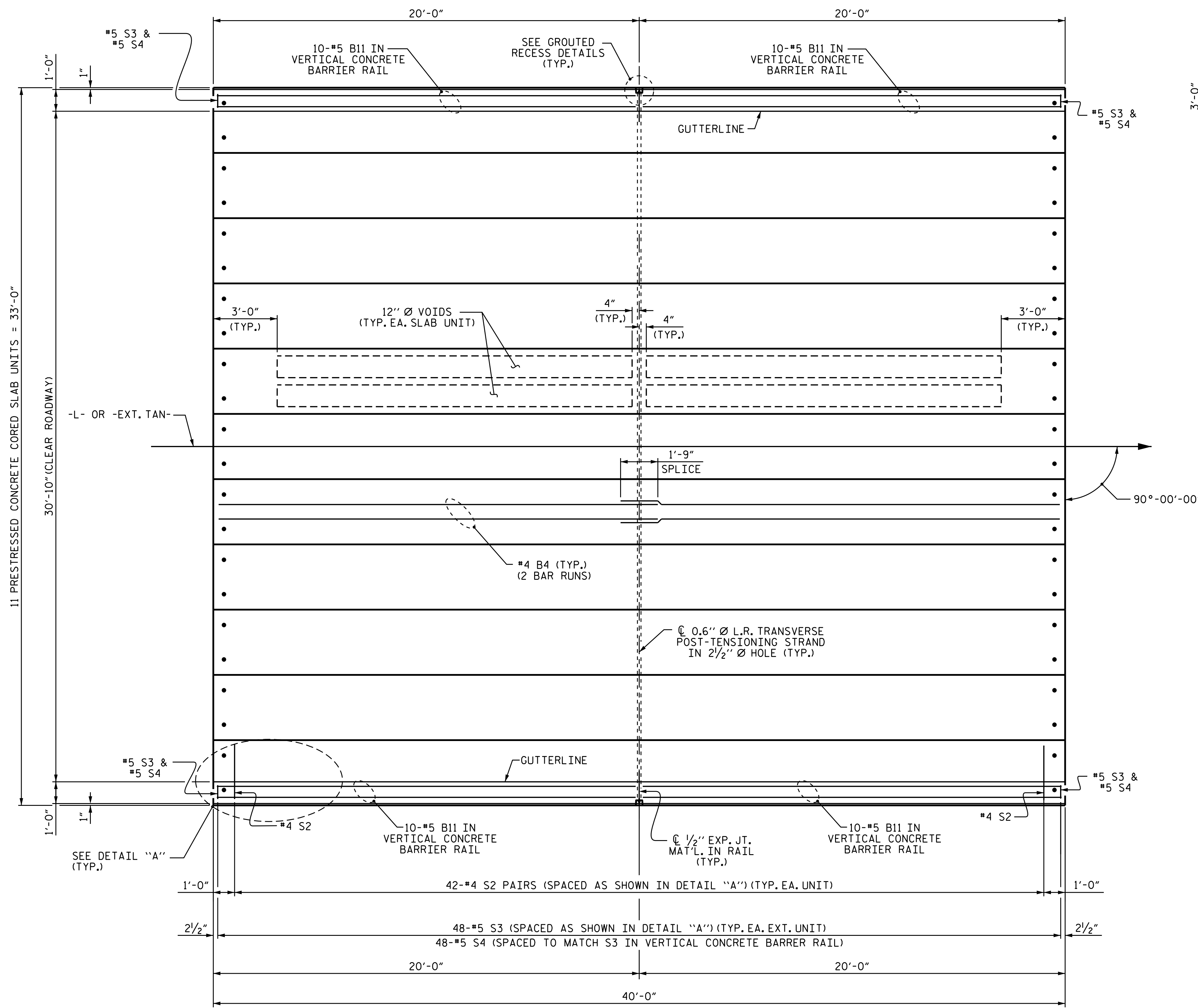
PLAN OF UNIT SPAN B
