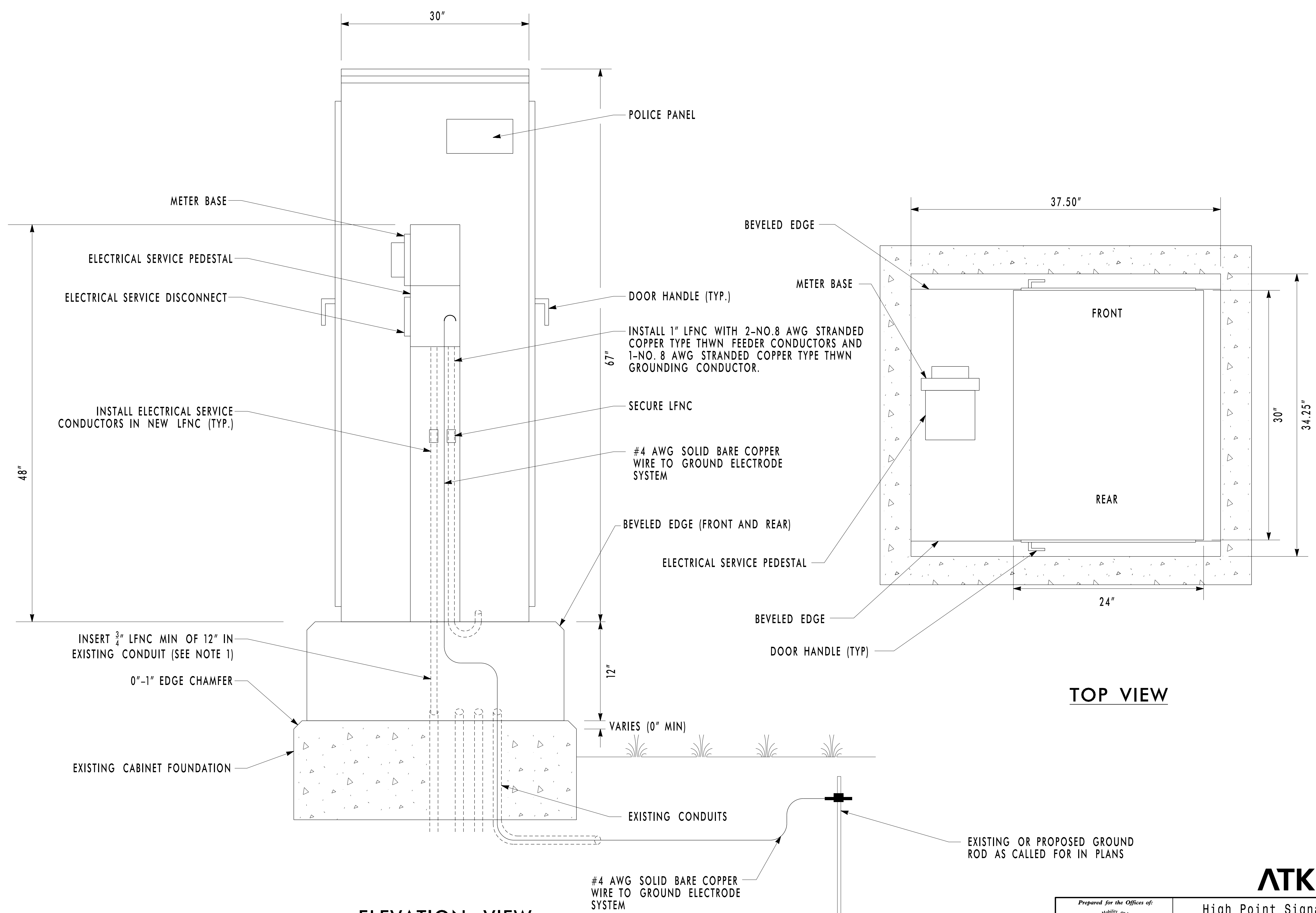
ELEVATION VIEW LEFT SIDE
