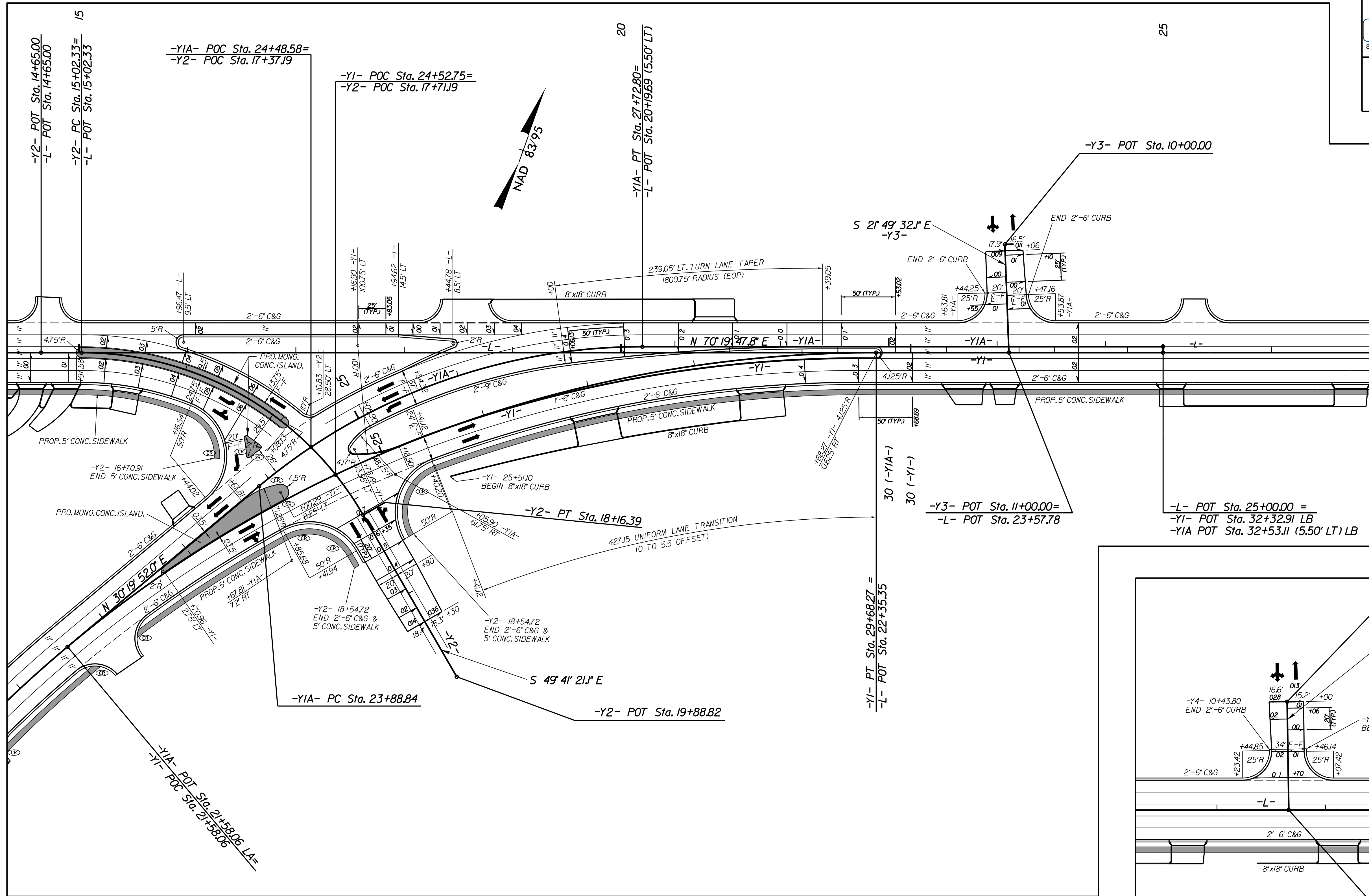
NC 268 (-Y1-/-Y1A-) ELKIN RD. / FLINT HILL RD. (-Y2-) INTERSECTION DETAIL SEE SHEET 4 FOR PLAN VIEW
