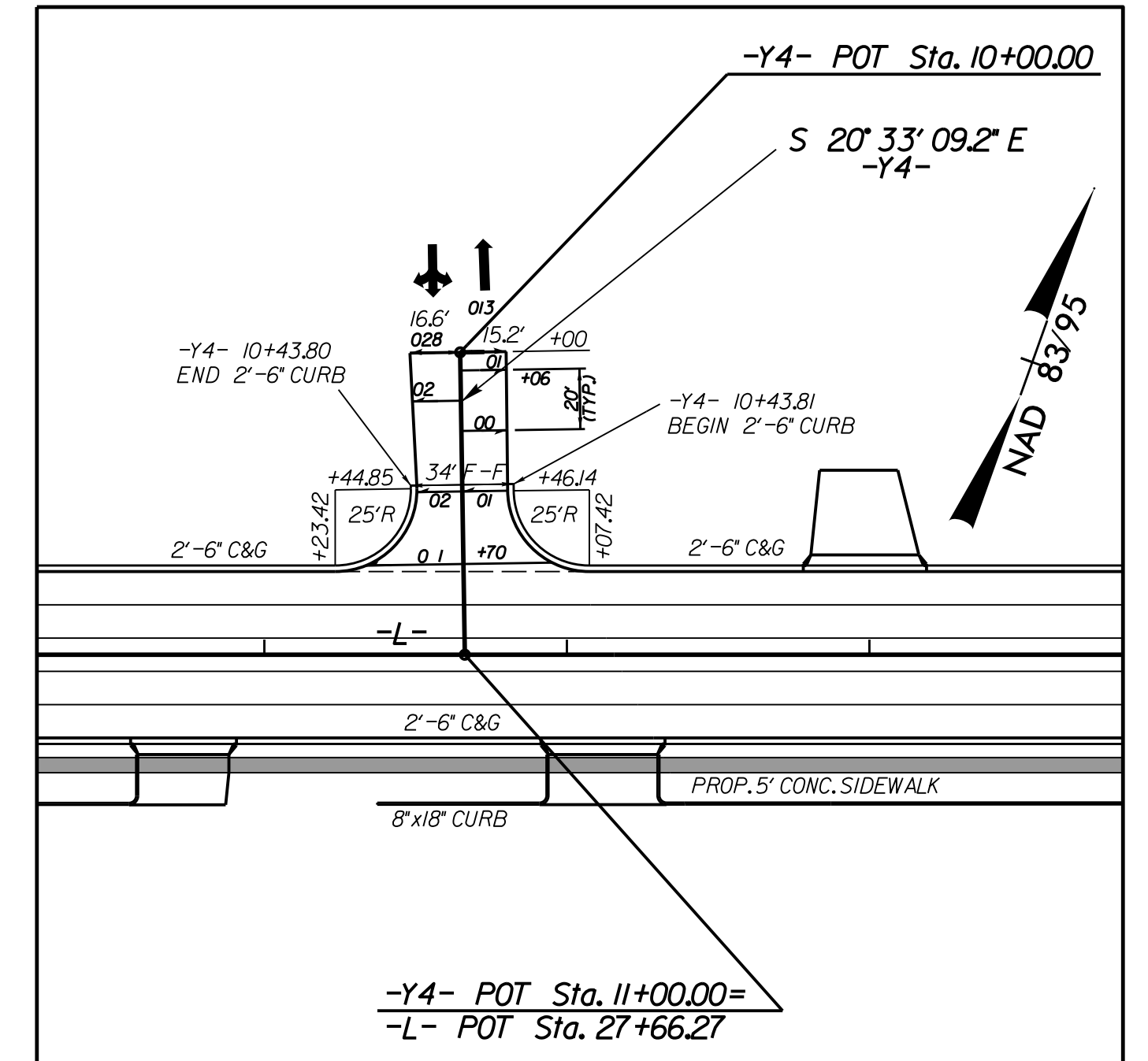
NC 268 (-L-) ELKIN RD. / TEMPLE ST. (-Y4-) INTERSECTION DETAIL SEE SHEET 5 FOR PLAN VIEW
