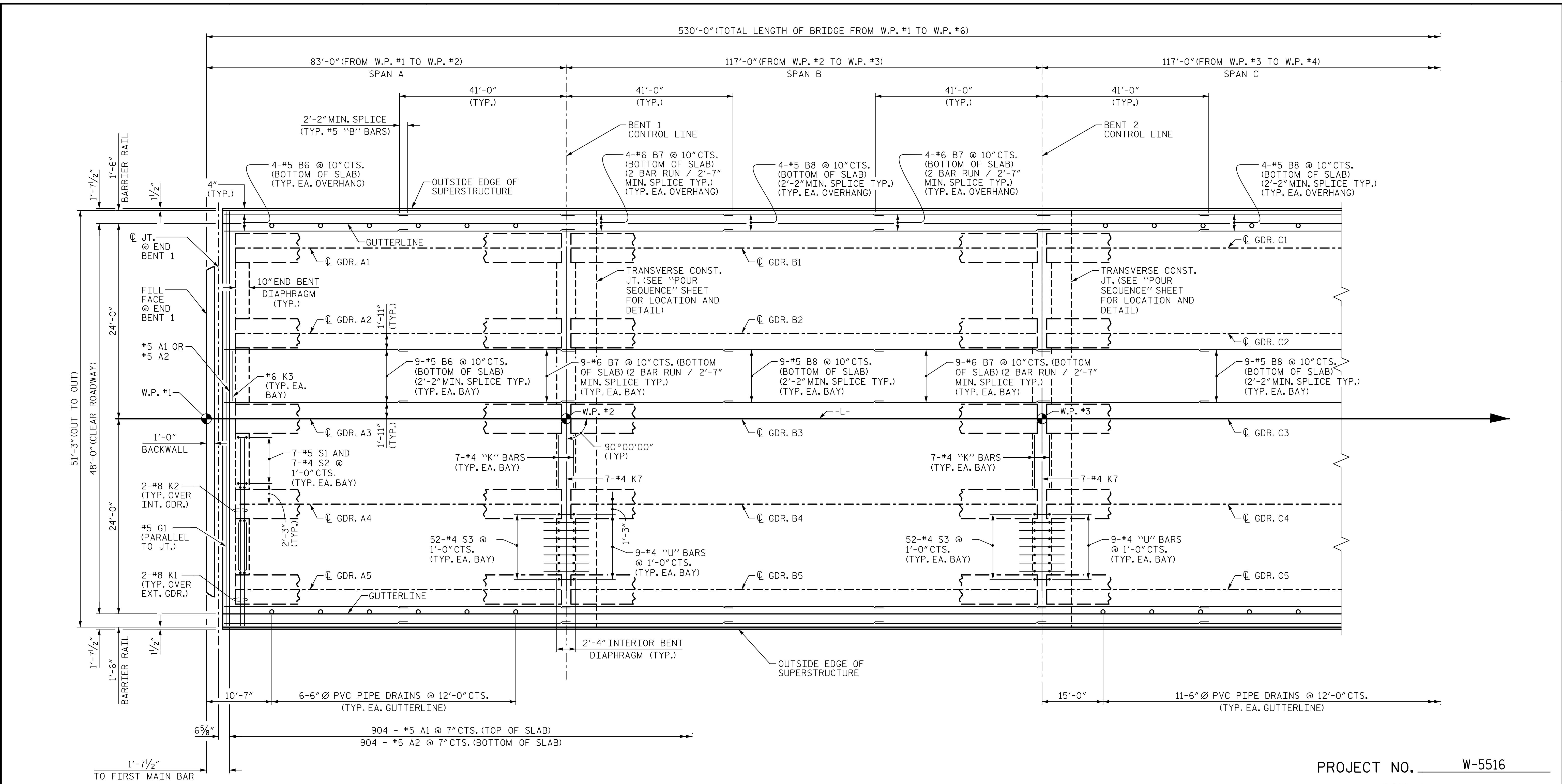
PARTIAL PLAN OF SPANS "A", "B" AND "C" FOR REINFORCING STEEL IN END BENT AND INTERIOR BENT DIAPHRAGMS, SEE "TYPICAL SECTION" SHEETS. FOR LONGITUDINAL BARS IN TOP OF SLAB, SEE SHT. 3 OF 4.
