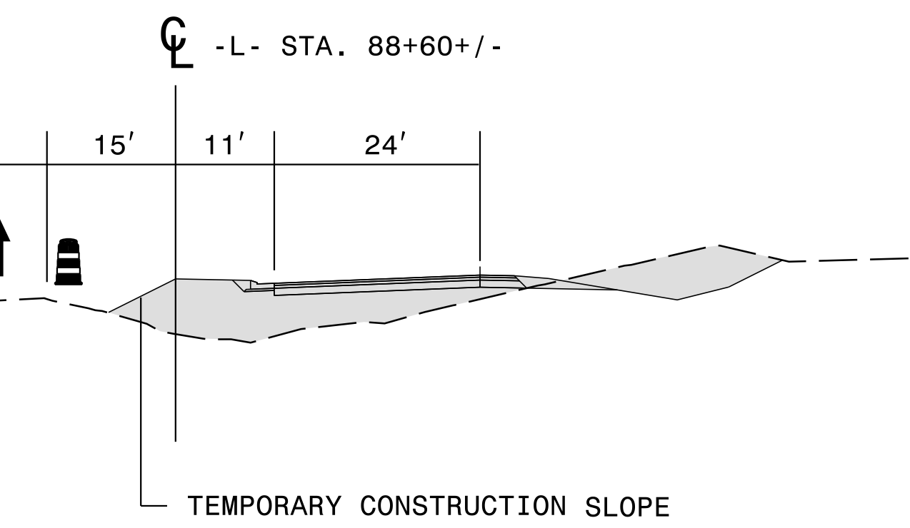
SECTION F-F
