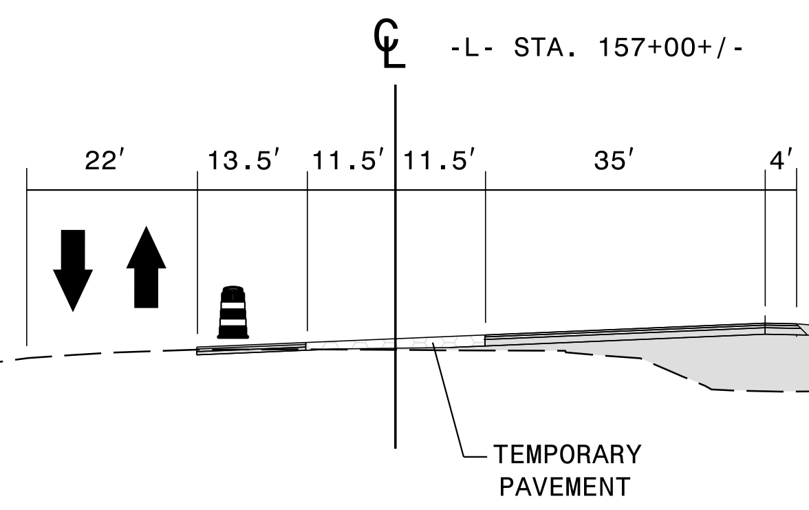
SECTION I-I
