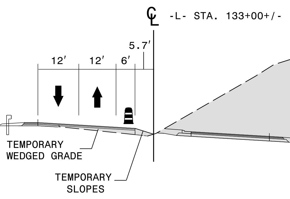
SECTION H-H
