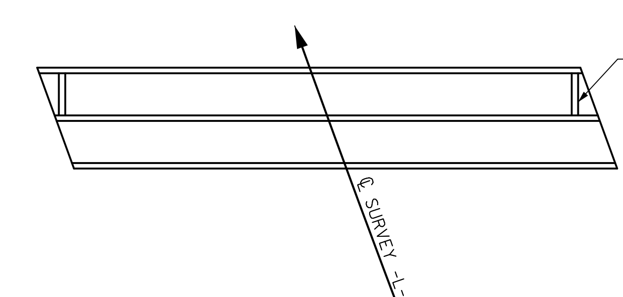
SILL LAYOUT PLAN
