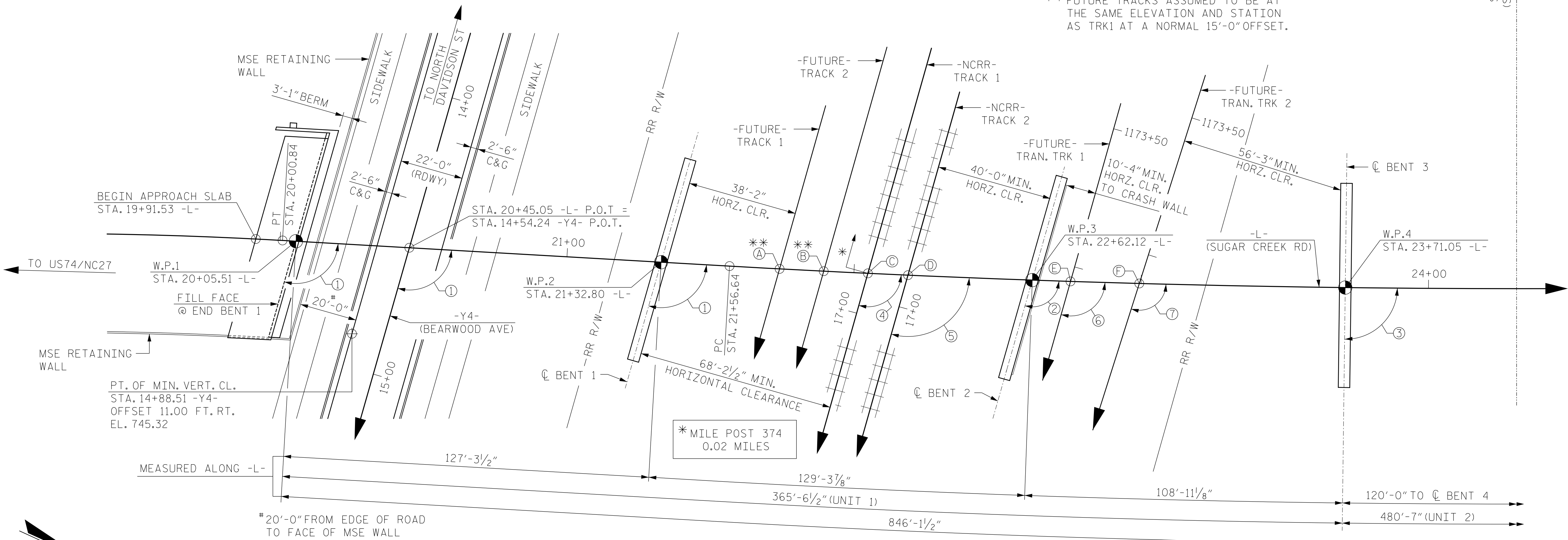
PLAN (PILES & DRILLED PIERS NOT SHOWN IN PLAN VIEW)
