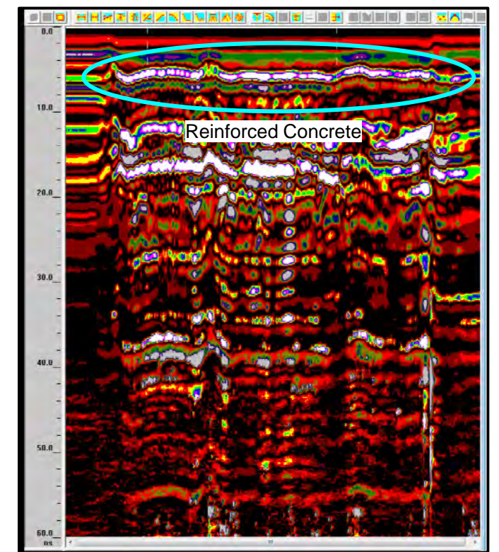
GPR Transect 1 - Example of Reinforced Concrete (No Evidence of any USTs observed)
