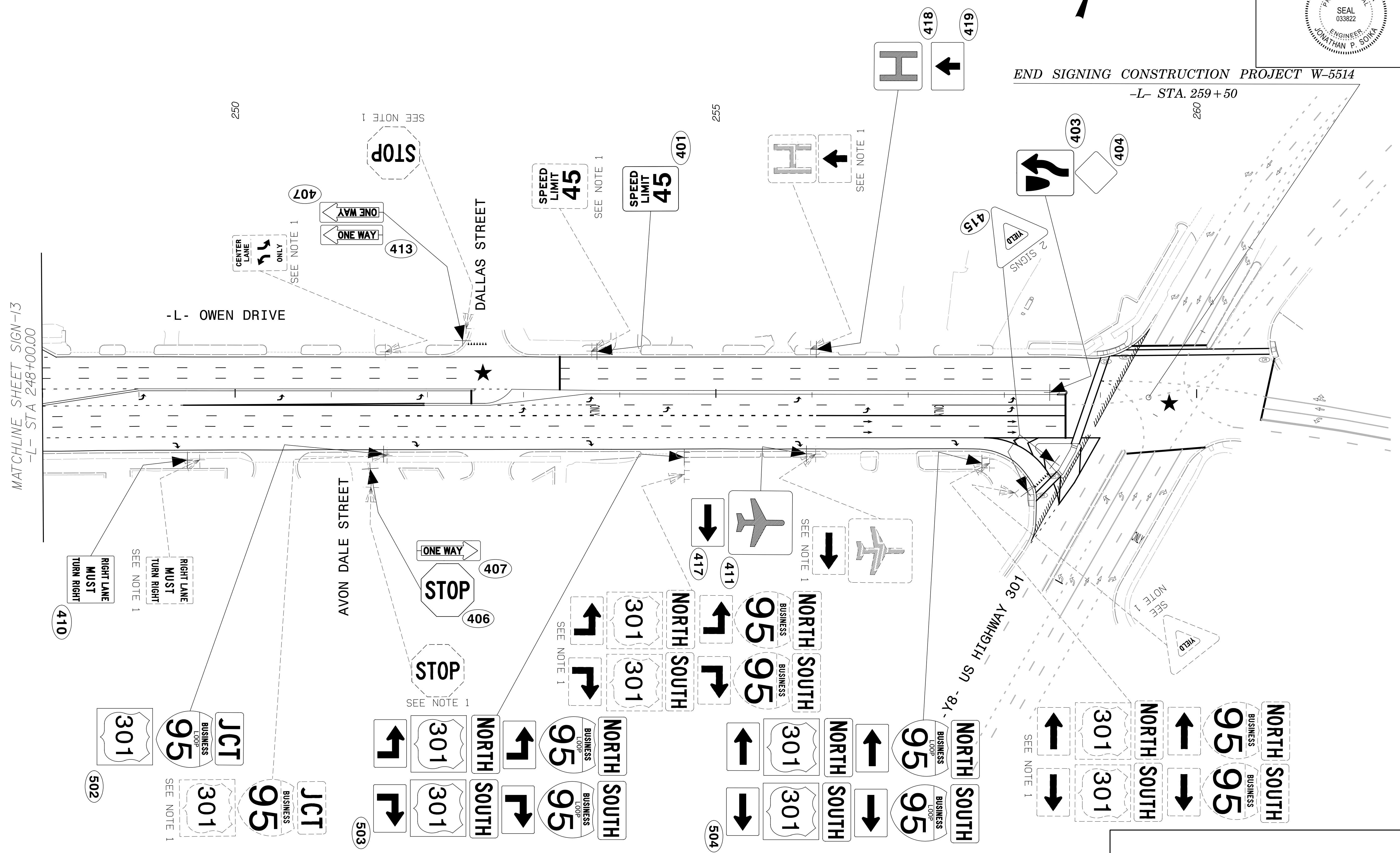
SIGNING DETAIL
