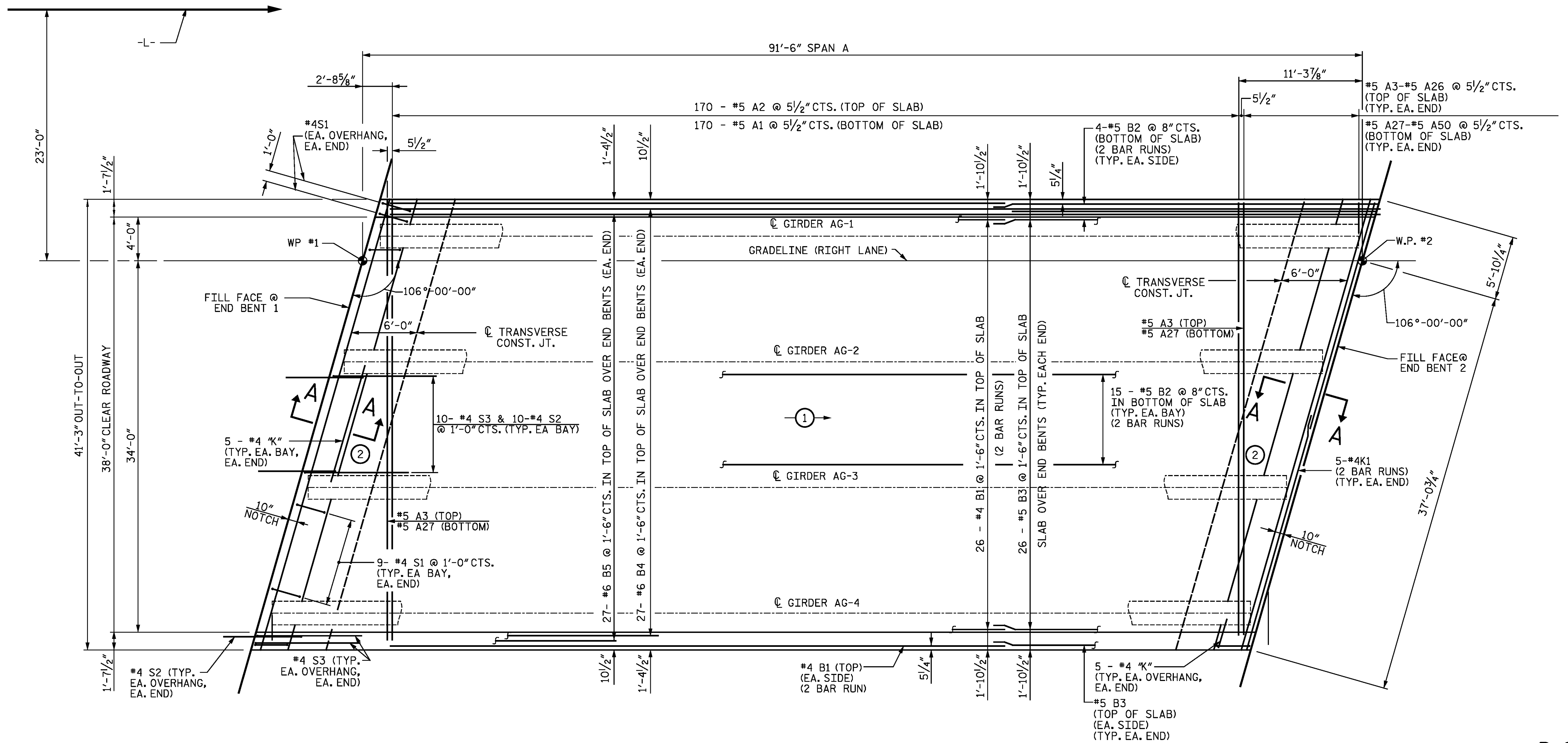
PLAN - SPAN A
