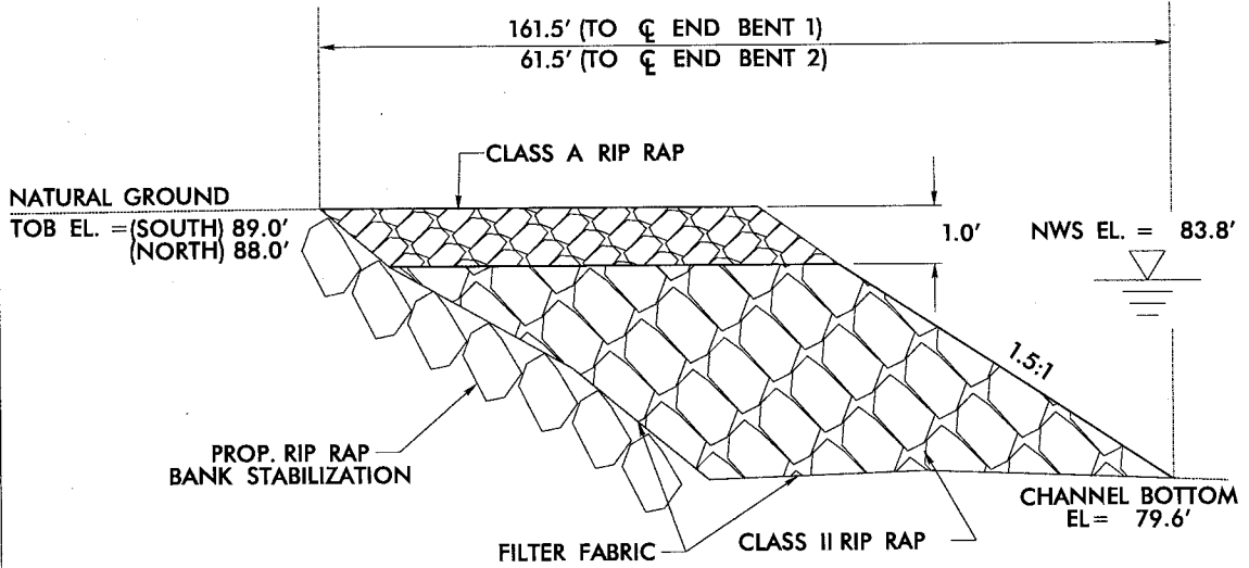
SECTION B-B
