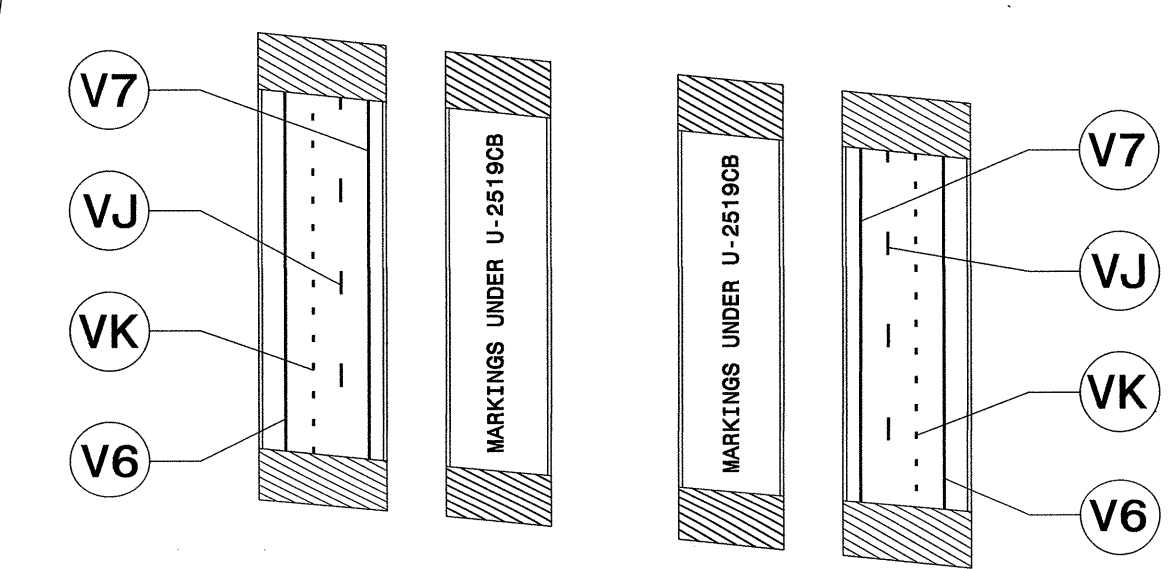
BRIDGE PAVEMENT MARKING DETAILS
