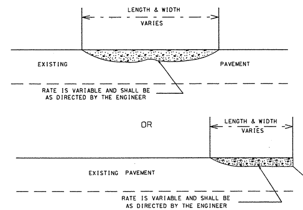
ASPHALT CONCRETE SURFACE COURSE TYPE S9.5B & SF9.5A (LEVELING COURSE)
