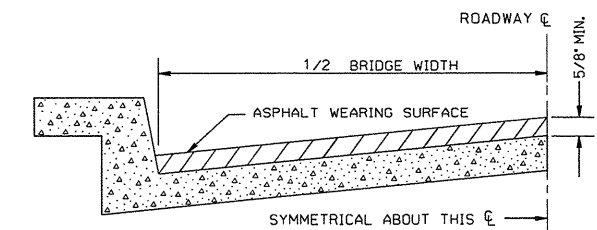
BRIDGE HALF TYPICAL SECTION
