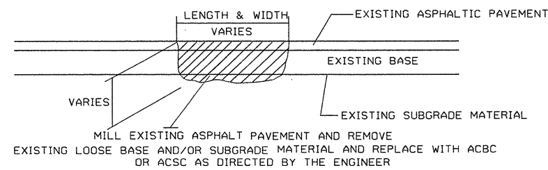
PATCHING EXISTING PAVEMENT
