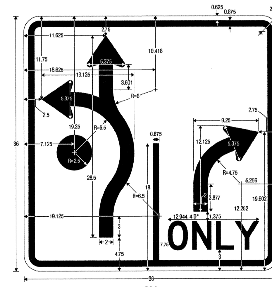
R3-8 ADVANCE CIRCULAR INTERSECTION LANE CONTROL - OPTIONAL, RIGHT TURN ONLY
