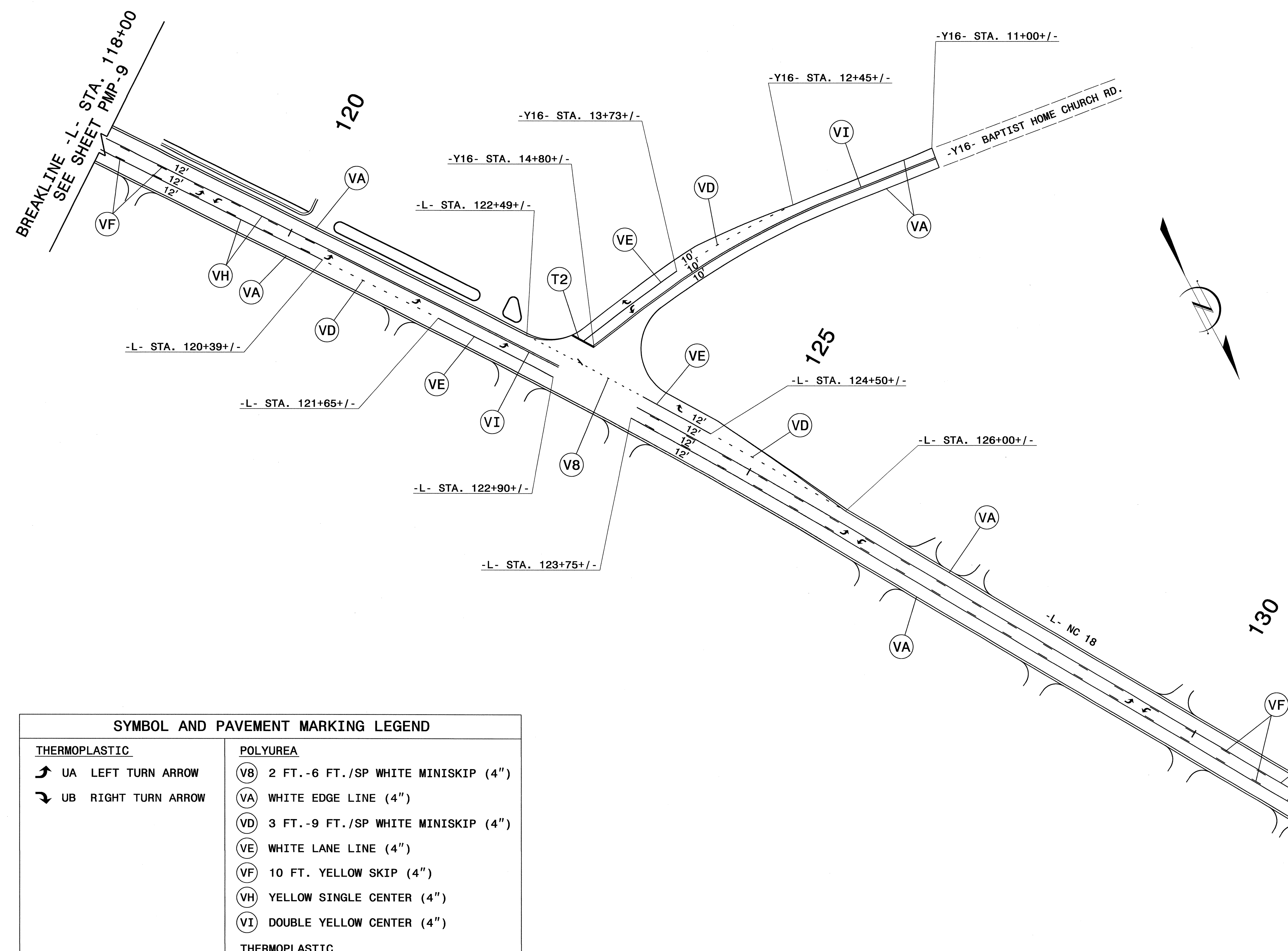
PAVEMENT MARKING DETAIL
