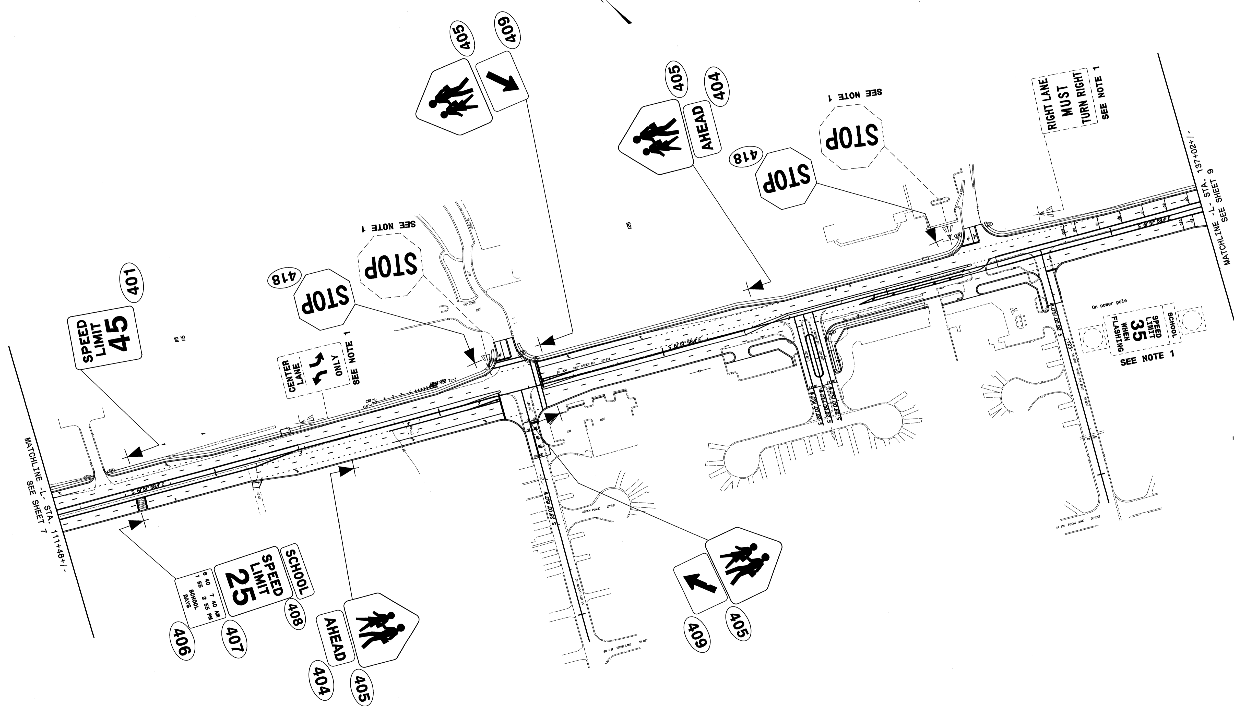
EXISTING & PROPOSED SIGNS -L- STA. 111+48+/- TO 137+02+/-
