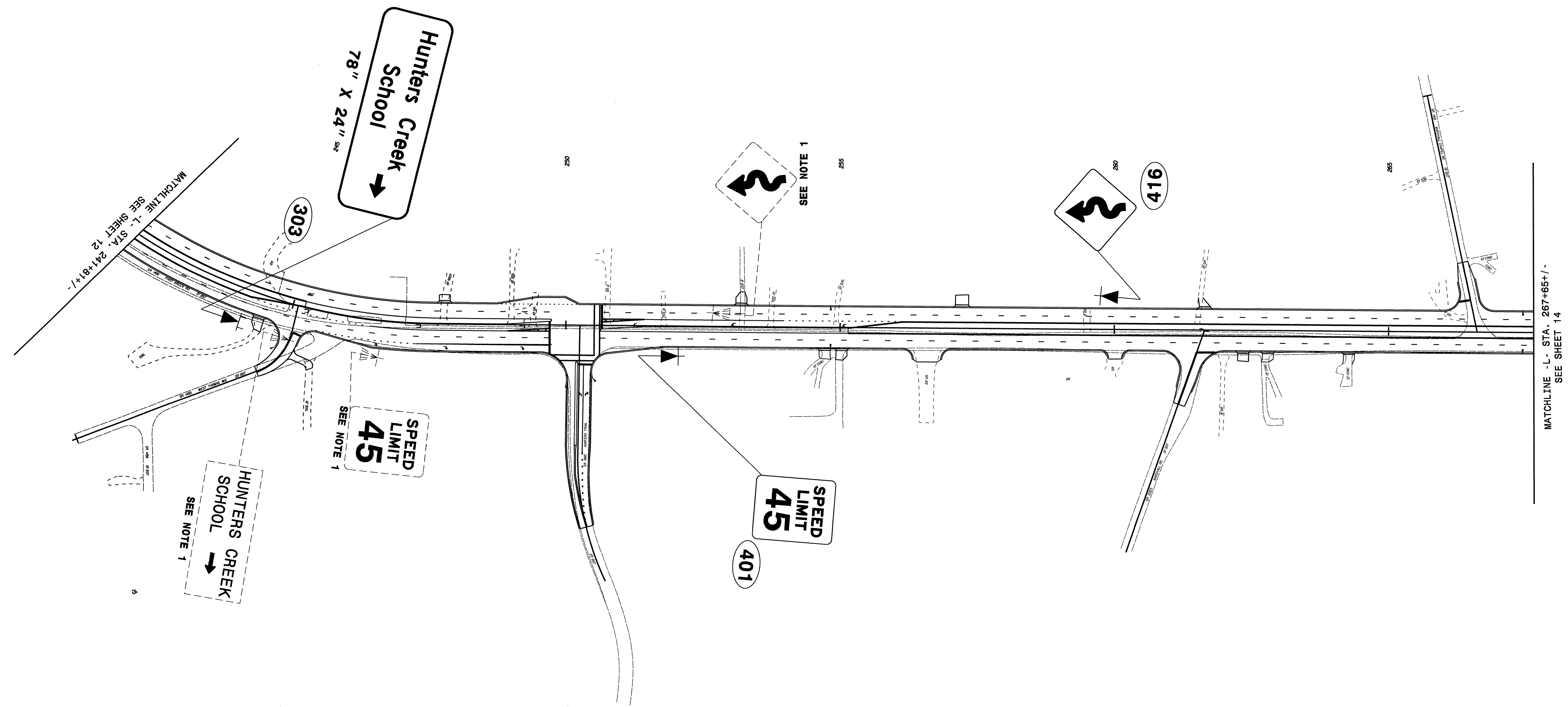
EXISTING & PROPOSED SIGNS -L-STA. 241+81+/- TO 267+65+/-
