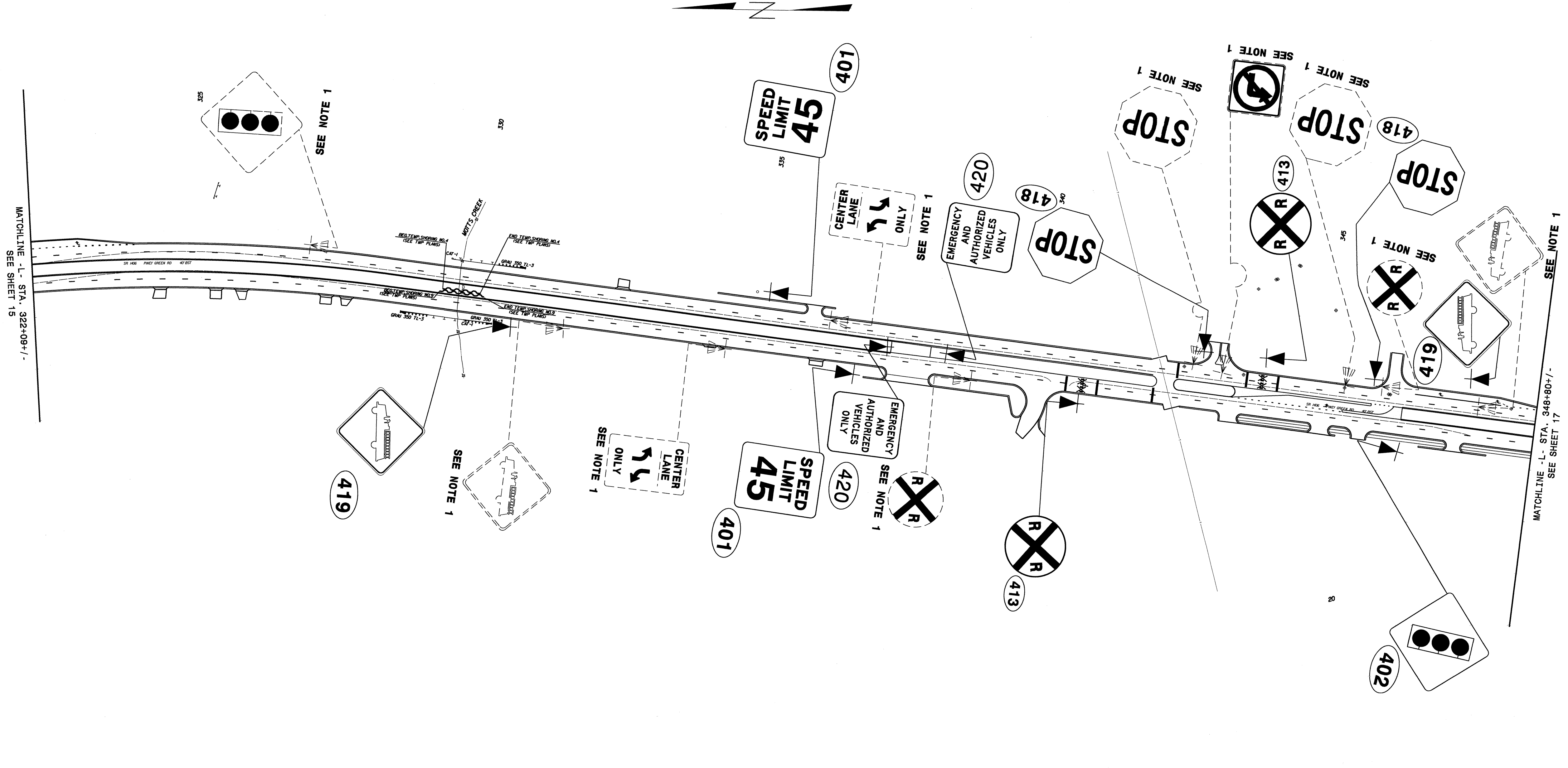
EXISTING & PROPOSED SIGNS -L- STA. 322+09+/- TO 348+80+/-
