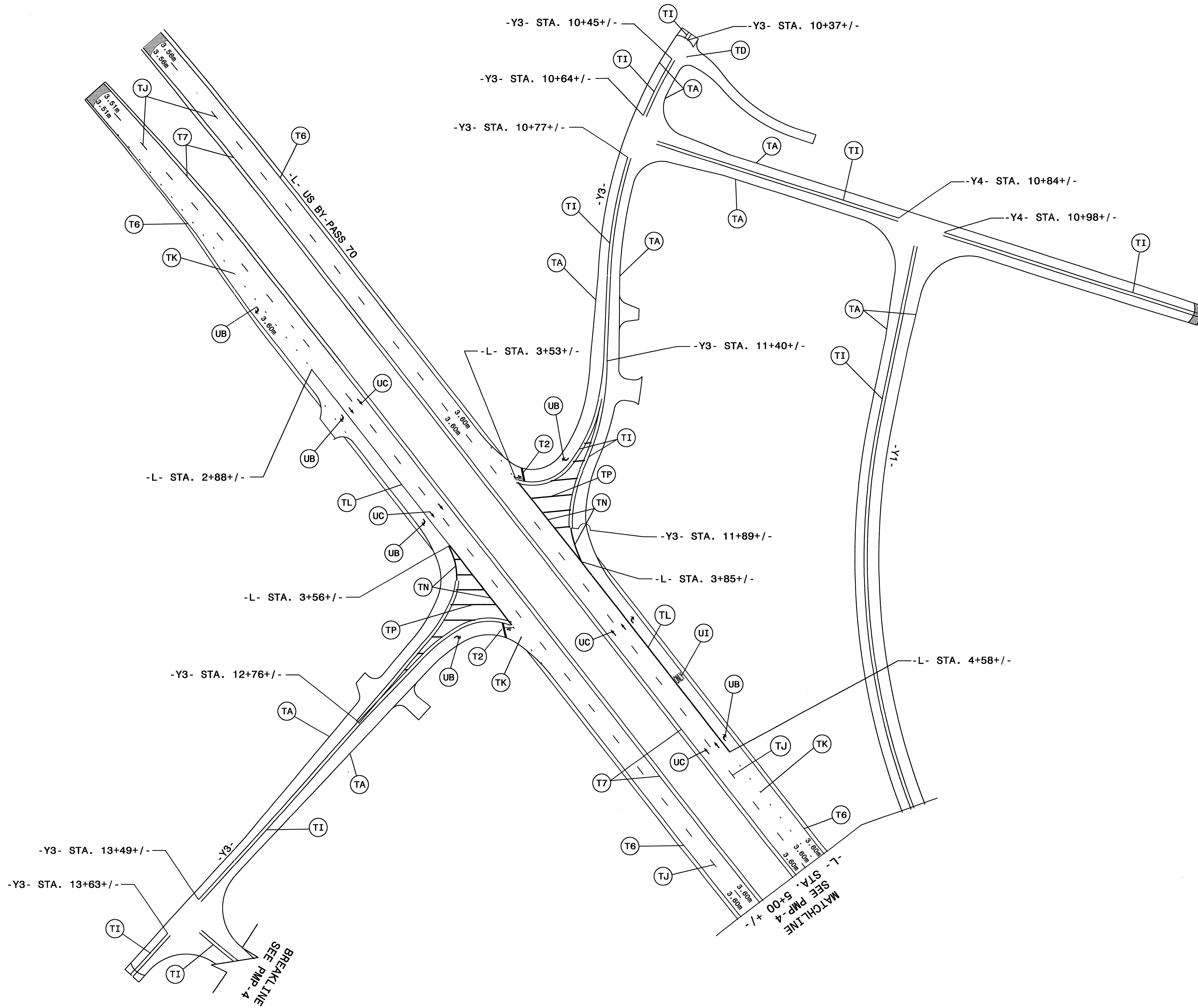
PAVEMENT MARKING DETAIL
