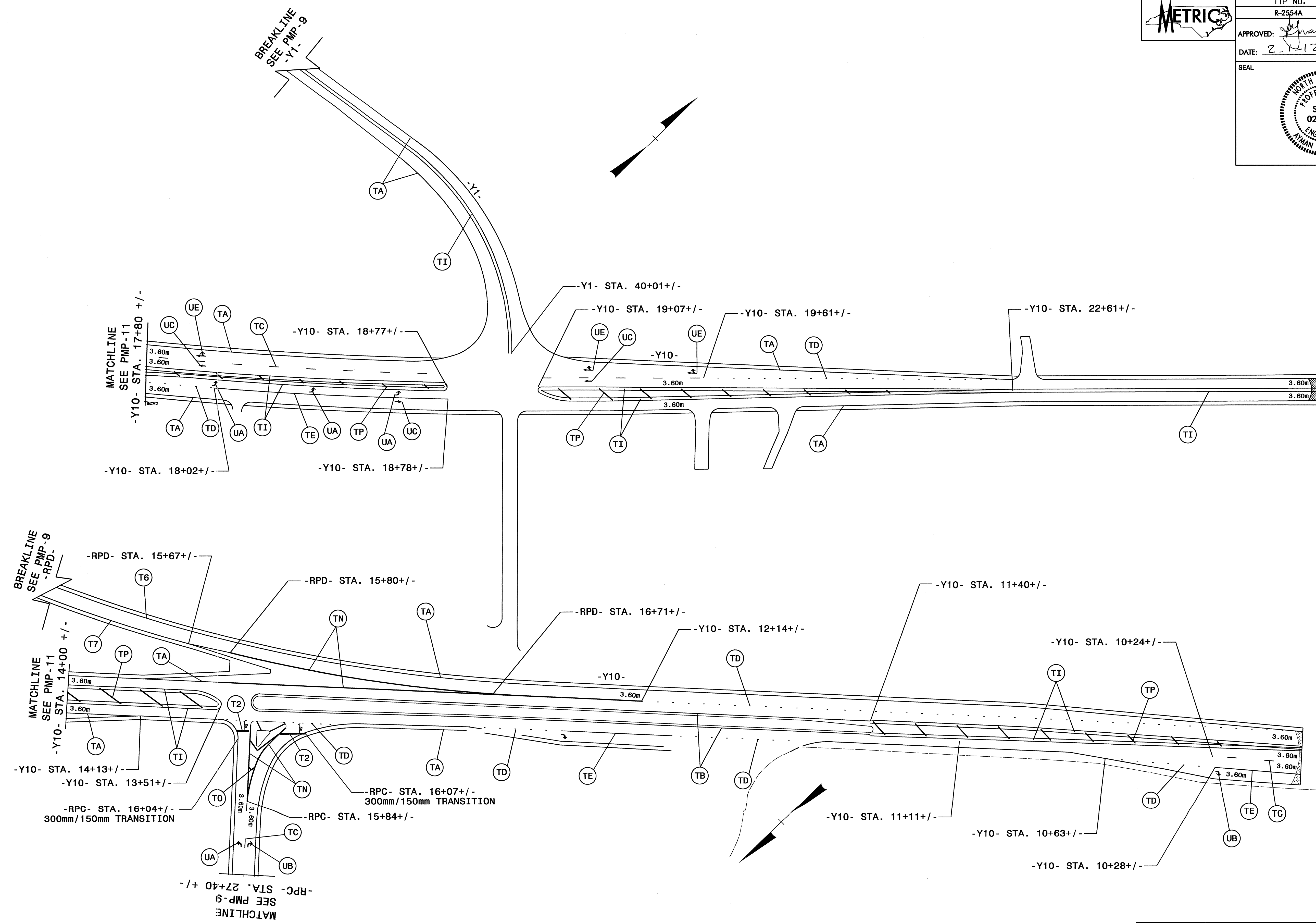
PAVEMENT MARKING DETAIL
