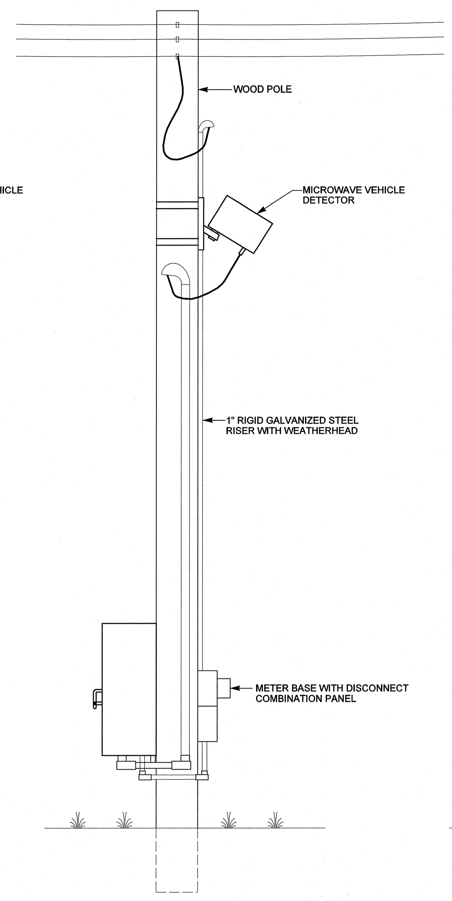
AERIAL ELECTRICAL SERVICE ON POLE
