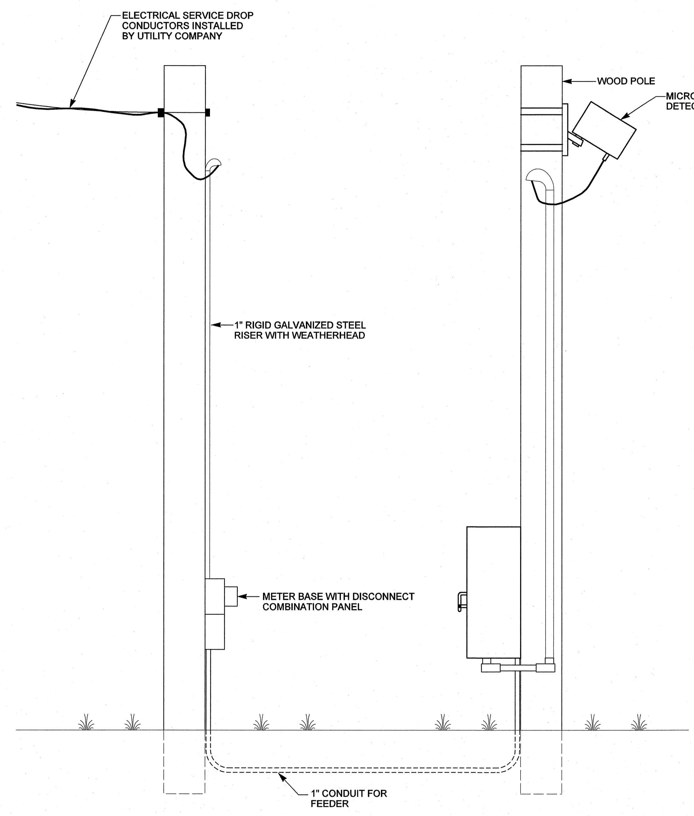
AERIAL ELECTRICAL SERVICE WITH SERVICE POLE
