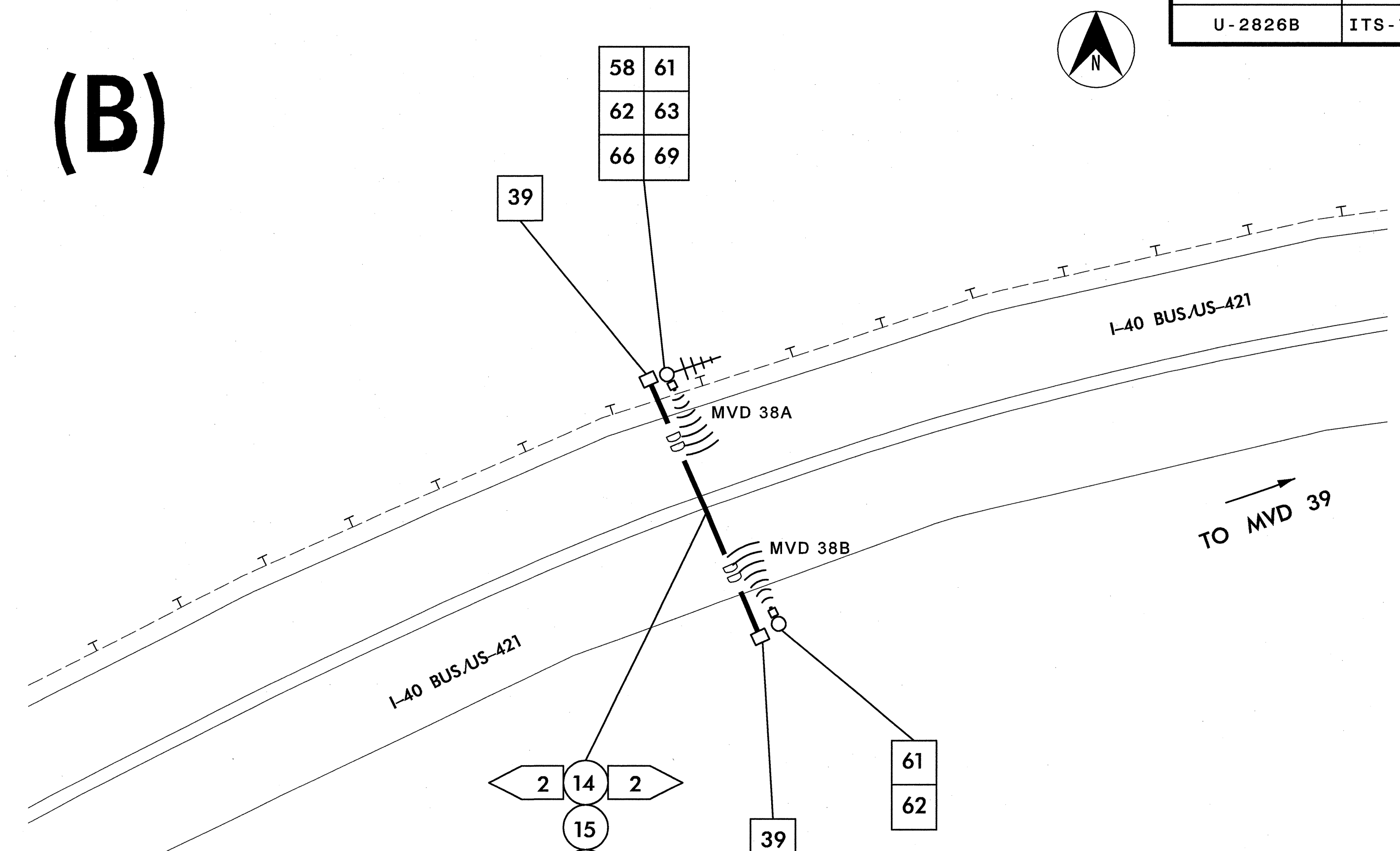
MVD 38: APPROXIMATELY 1100' WEST OF STRATFORD ROAD
