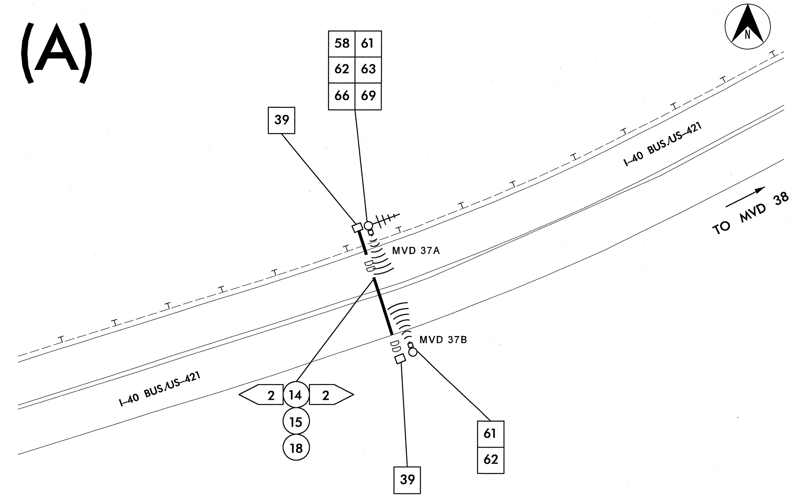
MVD 37: APPROXIMATELY 825' WEST OF WESTVIEW DRIVE
