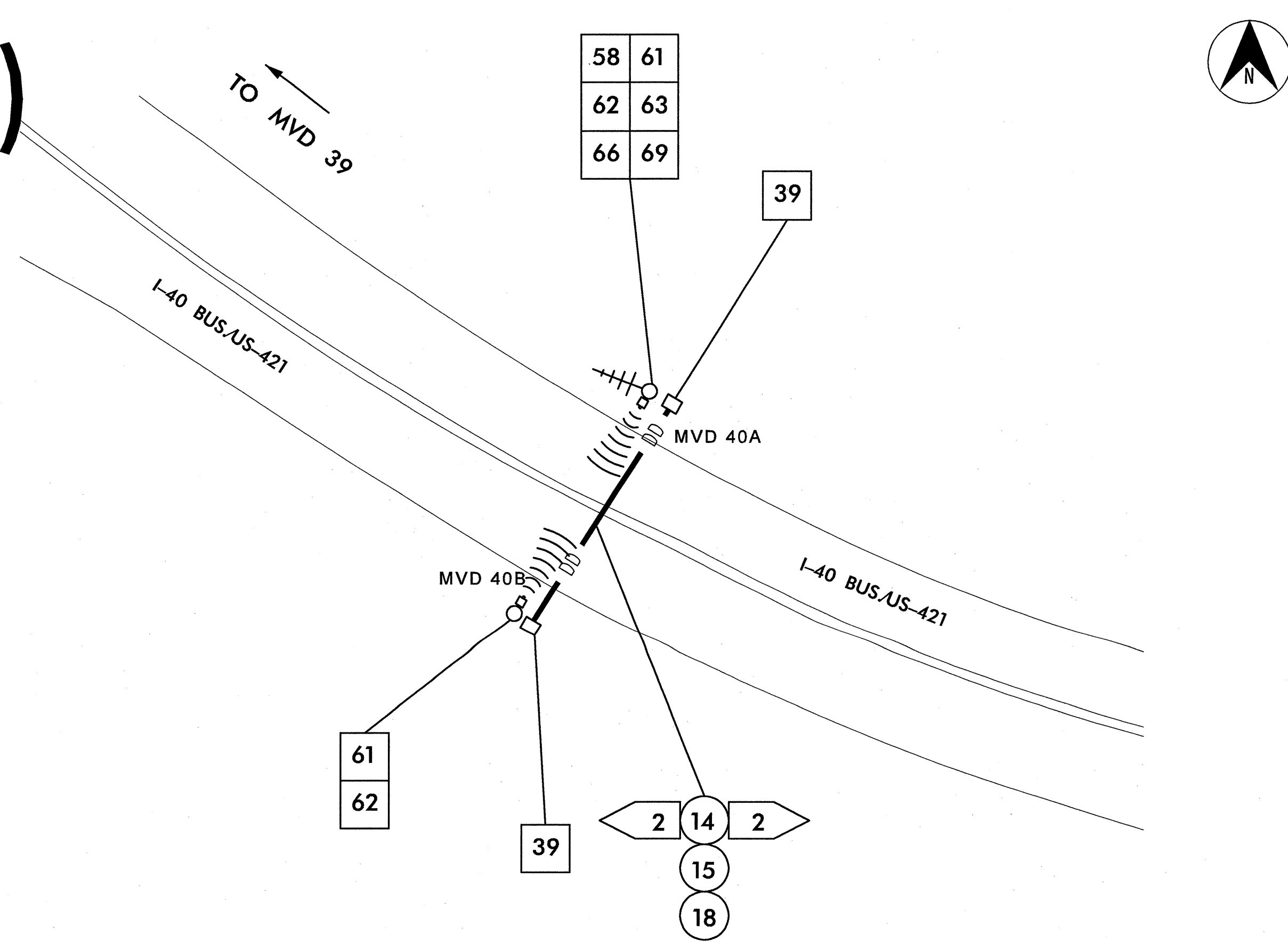
MVD 40: APPROXIMATELY 375' WEST OF CRAFTON STREET
