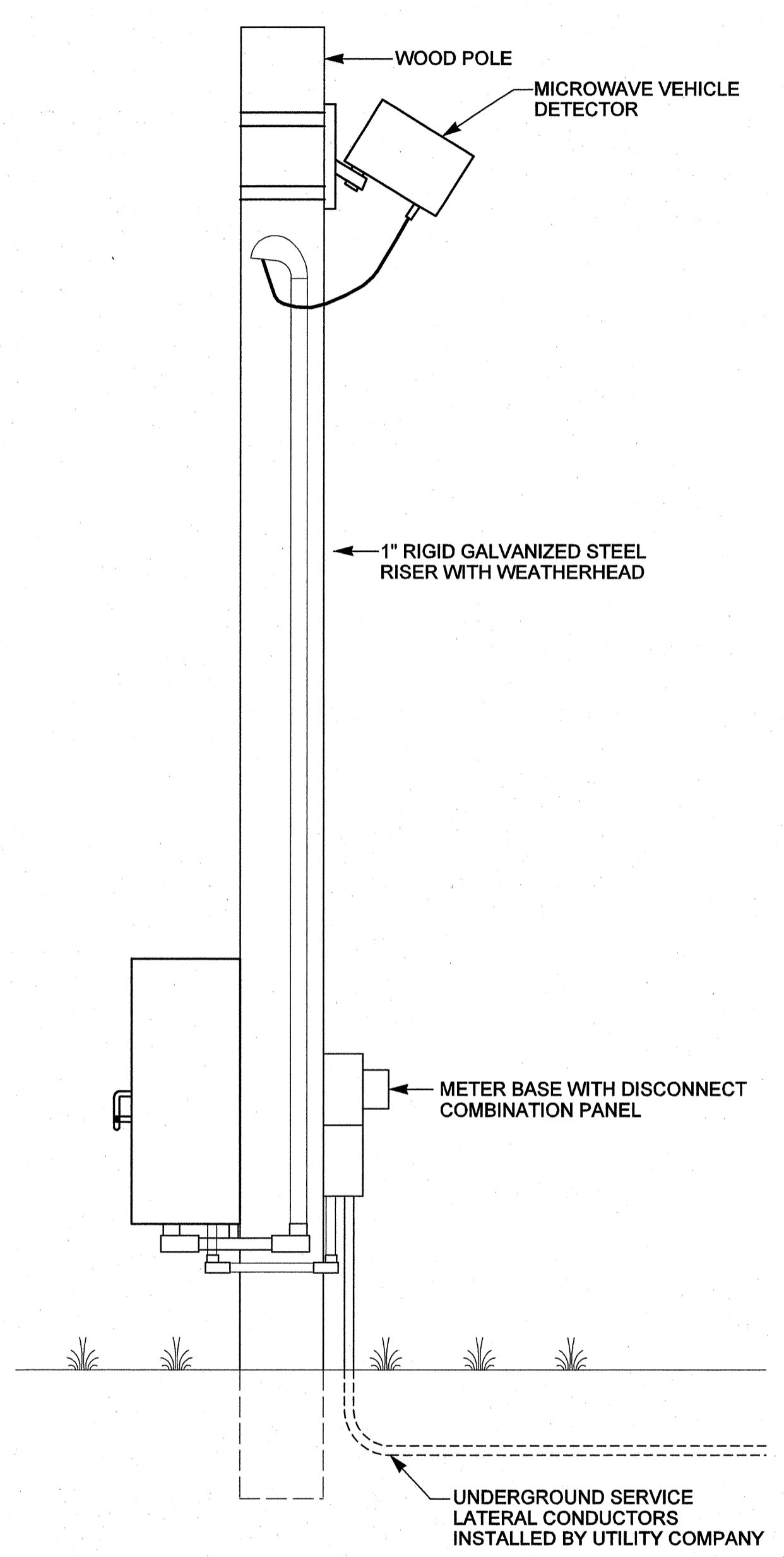
UNDERGROUND SERVICE
