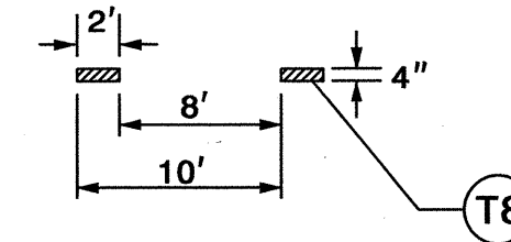
DETAIL 'C' MINI-SKIP SPACING FOR TURN LANES
