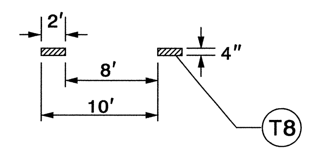
DETAIL 'A' SPECIAL DETAIL FOR MINI-SKIP SPACING FOR TURN AND BICYCLE LANES
