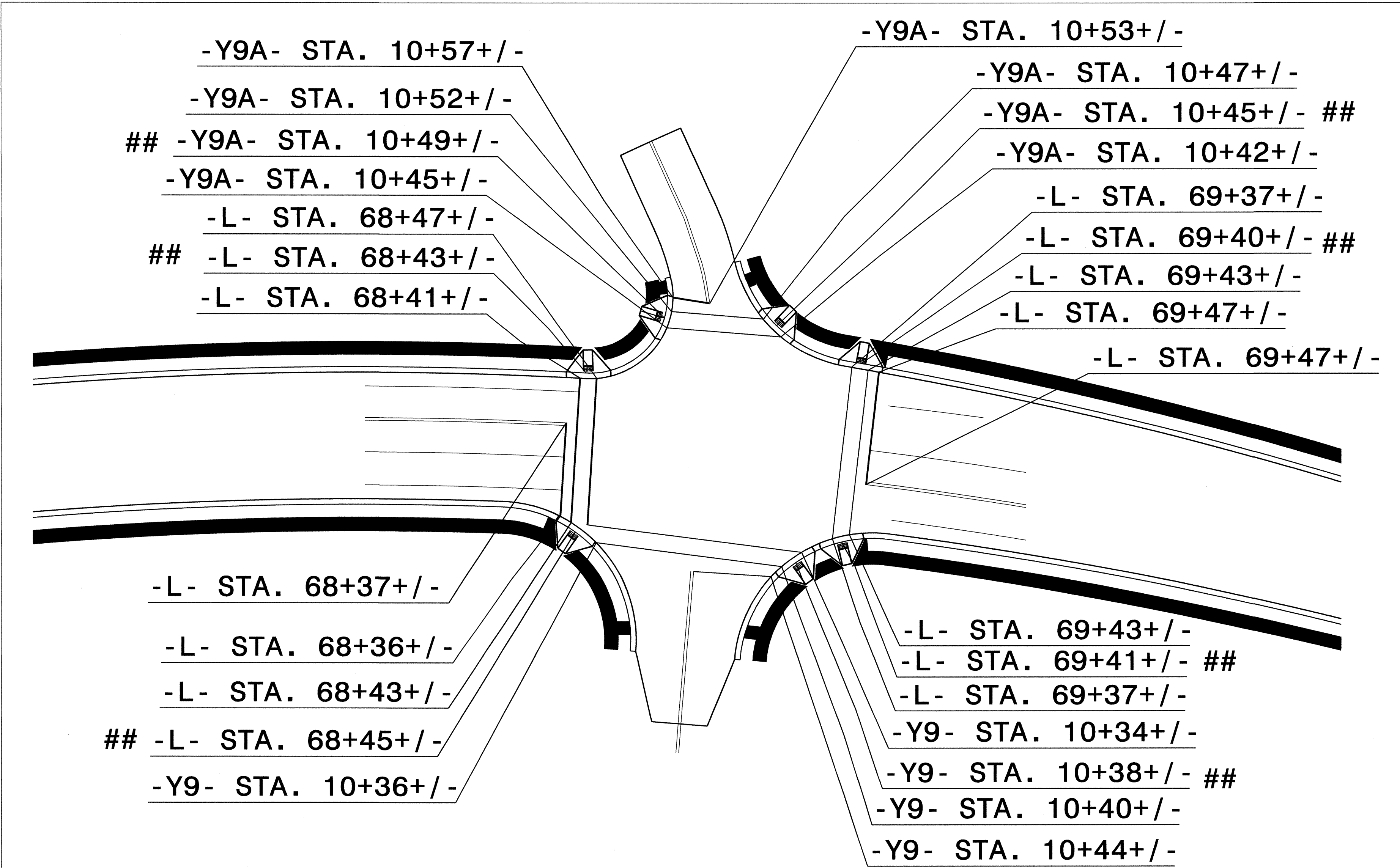
Stopbar and Crosswalk Locations For: SR 1733 (Weaver Diary Rd) at Silo Drive
