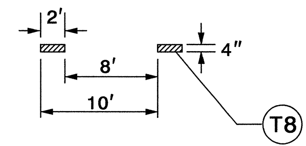
DETAIL 'A' SPECIAL DETAIL FOR MINI-SKIP SPACING FOR TURN AND BICYCLE LANES
