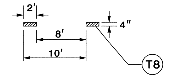
DETAIL 'A' SPECIAL DETAIL FOR MINI-SKIP SPACING FOR TURN AND BICYCLE LANES
