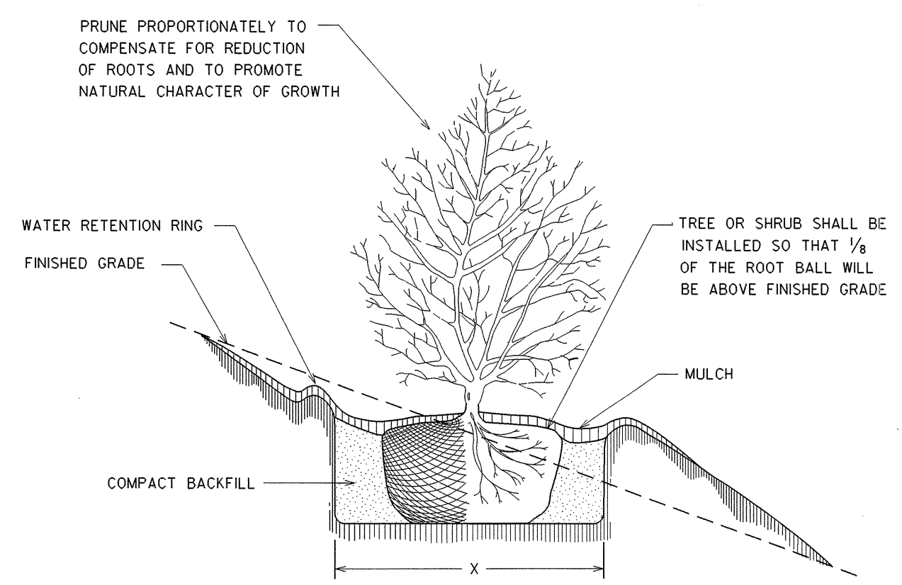
TREE OR SHRUB PLANTING DETAIL (SLOPING GROUND)
