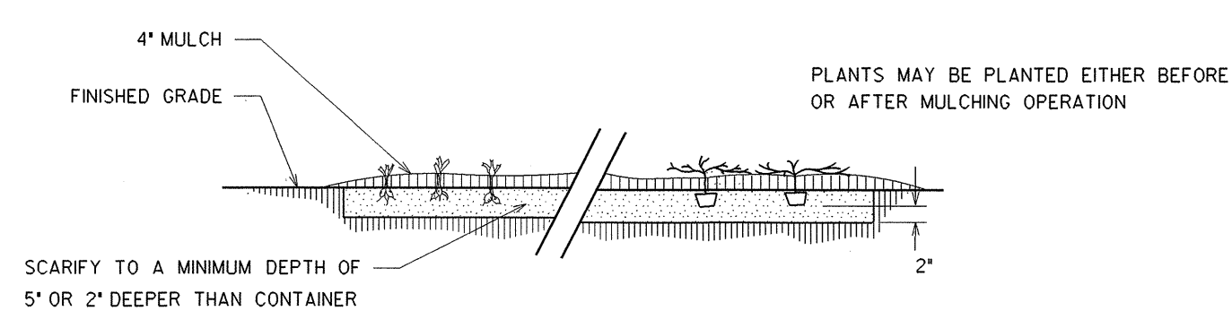
GROUNDCOVER PLANTING DETAIL
