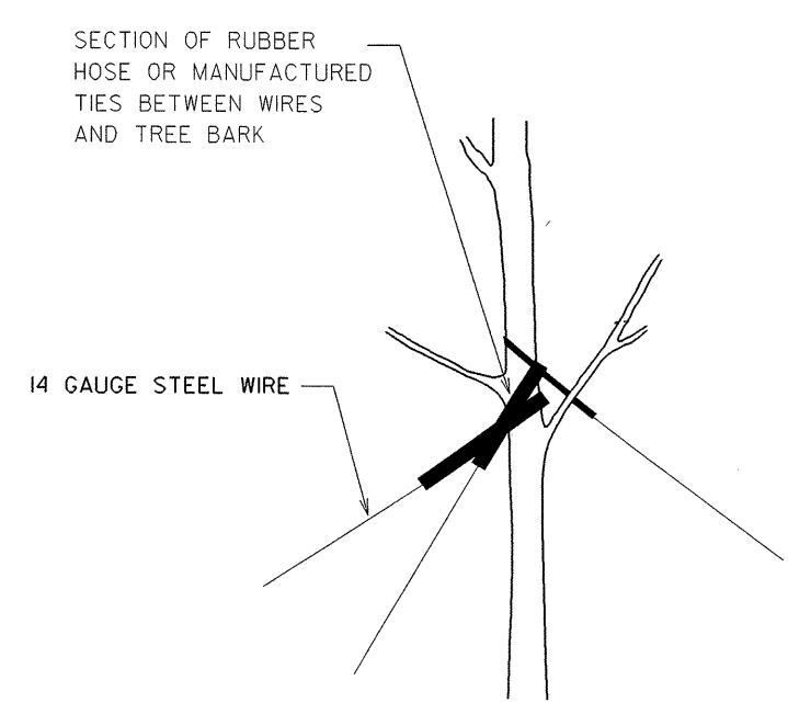
GUY TYING DETAIL
