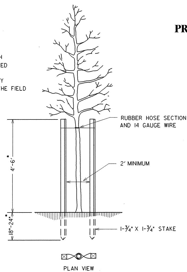
STAKING DETAIL (FOR TREES 6' TO 10')
