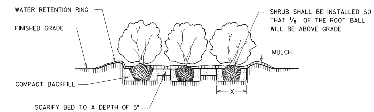
SHRUB BED PLANTING DETAIL
