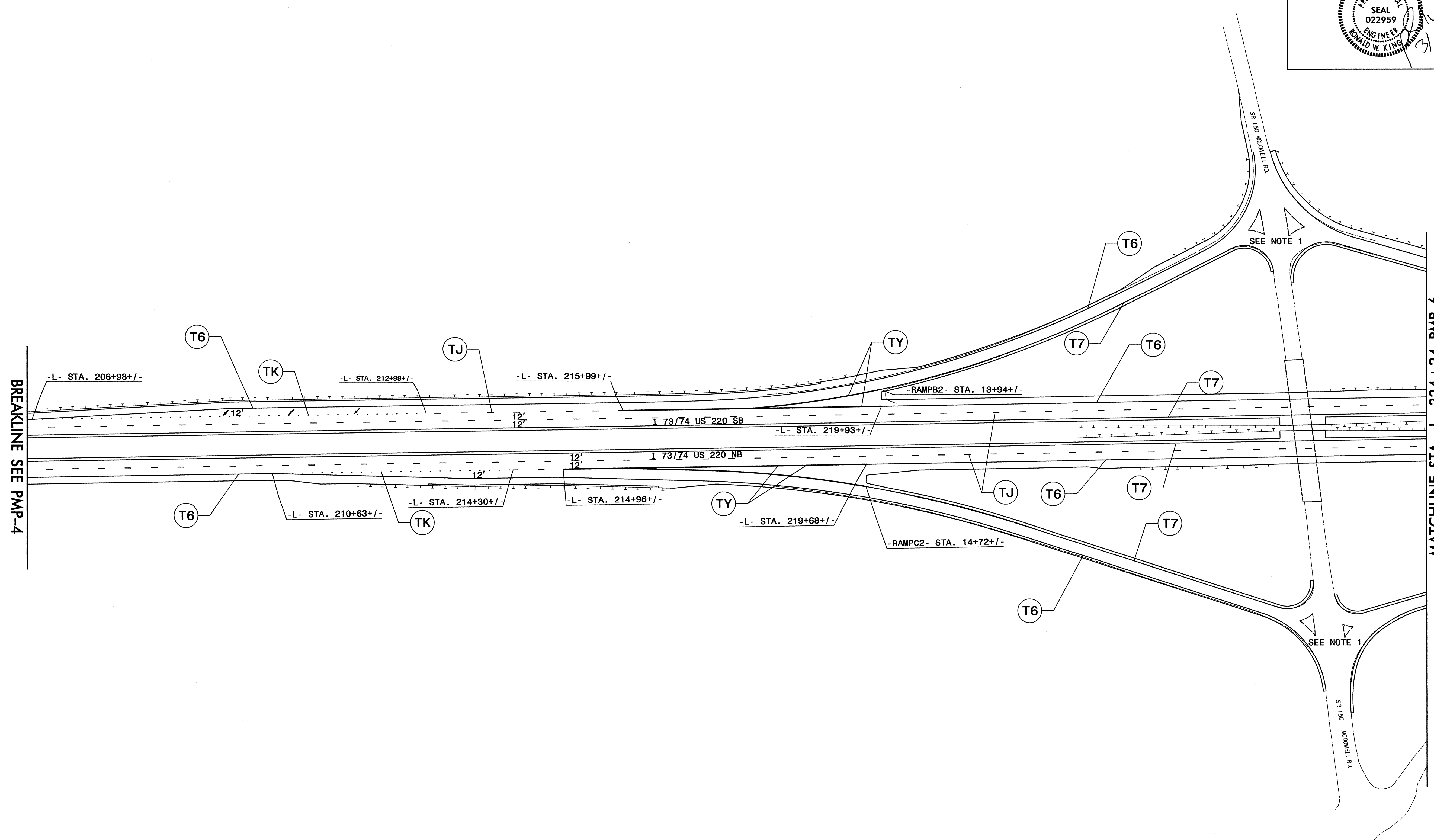
PROPOSED PAVEMENT MARKING PLANS
