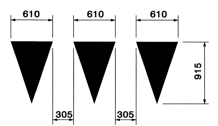
SPECIAL DETAIL FOR YIELD LINE SHARK TEETH - UJ PAYMENT FOR YIELD LINE SHARK TEETH WILL BE BASED ON THERMOPLASTIC SYMBOL (2.3mm) (ALL DIMENSIONS ARE IN MM)
