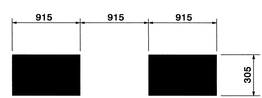
SPECIAL DETAIL FOR YIELD LINE MINISKIP - T8 PAYMENT FOR YIELD LINE MINISKIP WILL BE BASED ON THERMOPLASTIC (600mm, 3.1mm) (ALL DIMENSIONS ARE IN MM)
