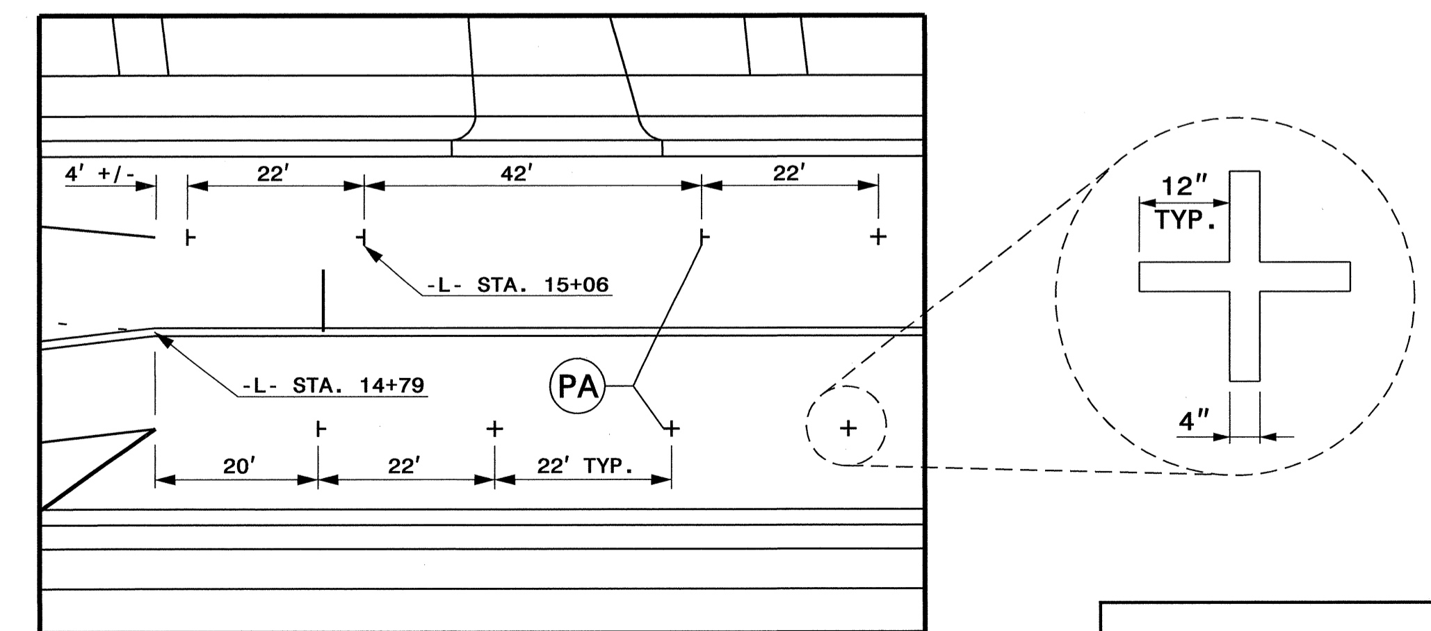
PAVEMENT MARKING DETAIL
