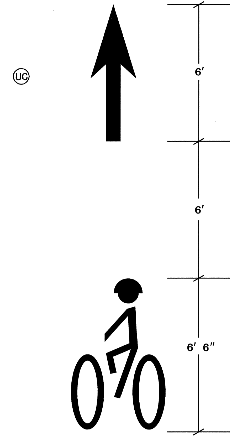
SPECIAL DETAIL FOR BIKE SYMBOL (UJ/UC)
