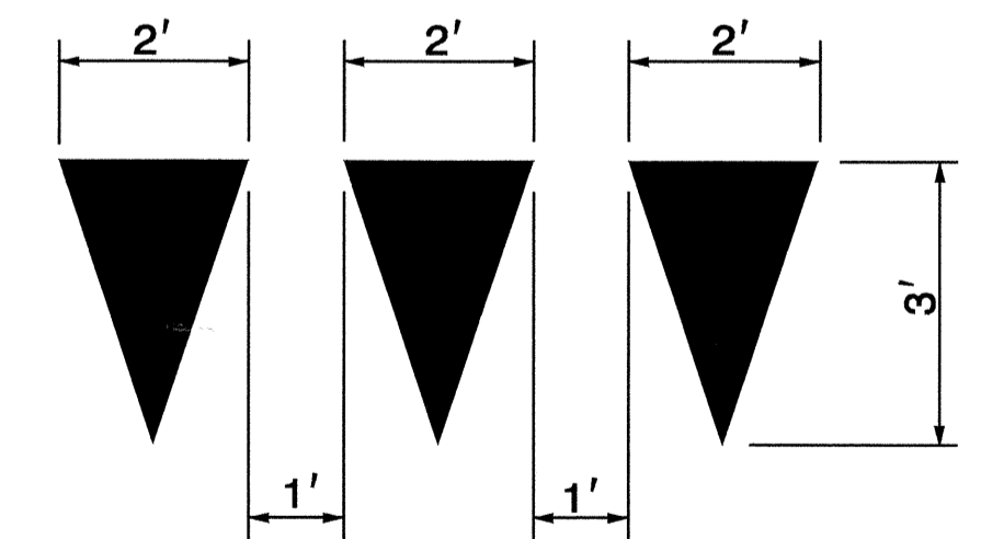
SPECIAL DETAIL FOR YIELD LINE SHARK TEETH - (UM)
