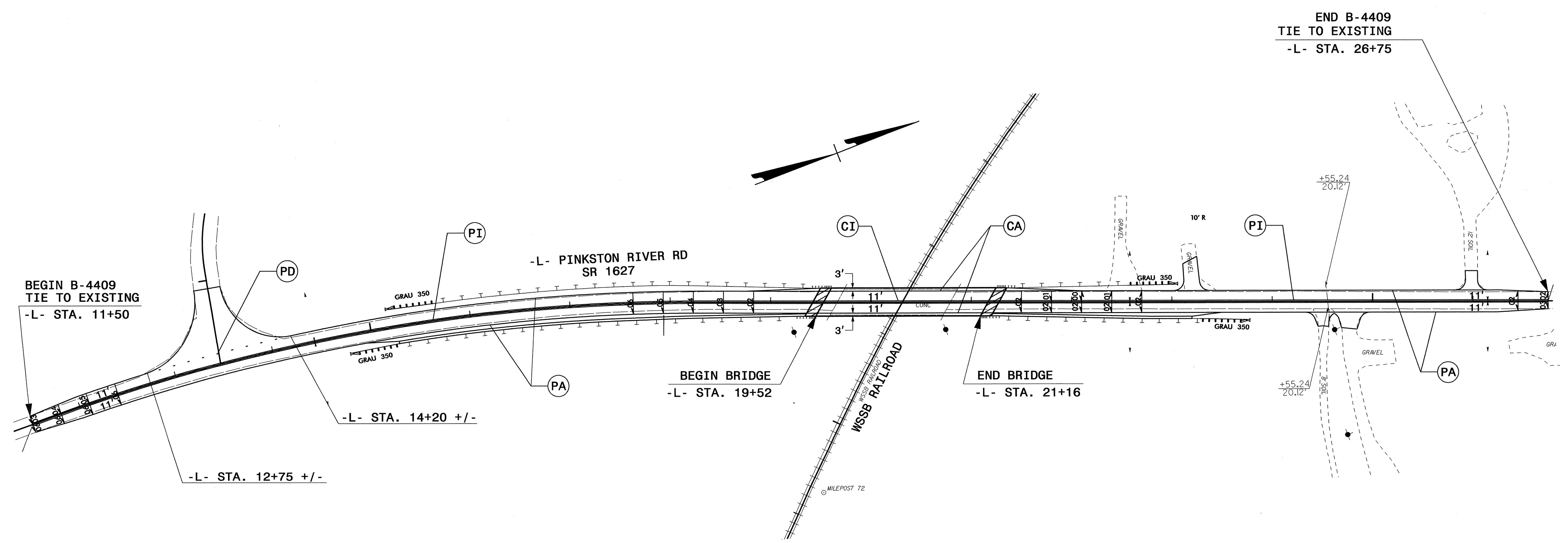
FINAL PAVEMENT MARKING SCHEDULE AND PAVEMENT MARKING DETAIL
