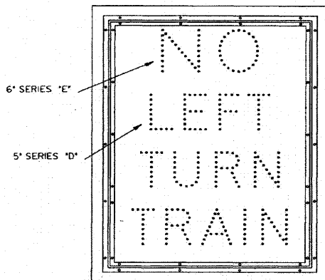
MESSAGE NO LEFT TURN TRAIN • SINGLE STROKE MESSAGE • WHITE LED'S
