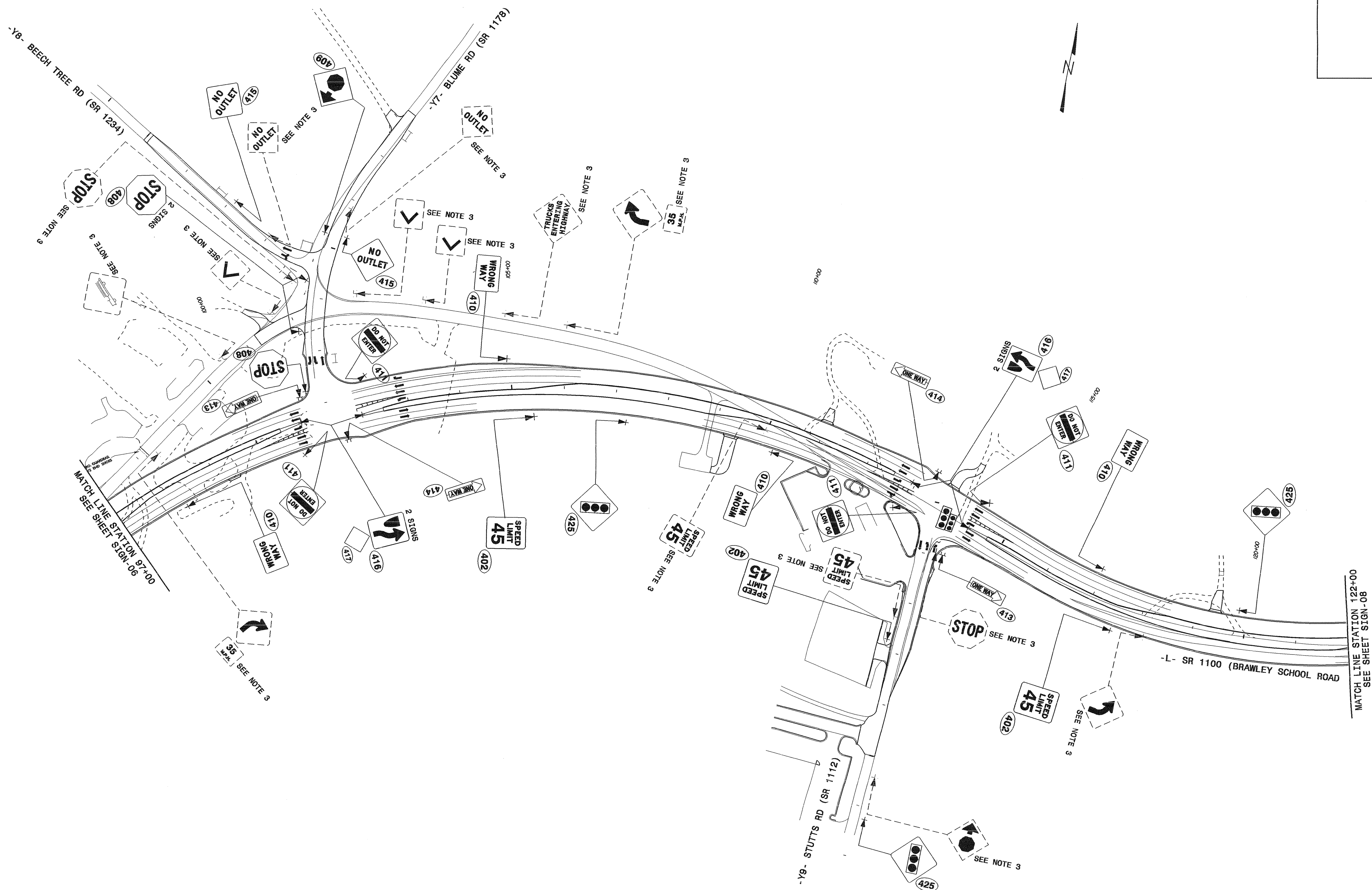
EXISTING AND PROPOSED SIGNS -L- STA. 97+00 TO 122+00 SR 1100 (BRAWLEY SCHOOL RD)
