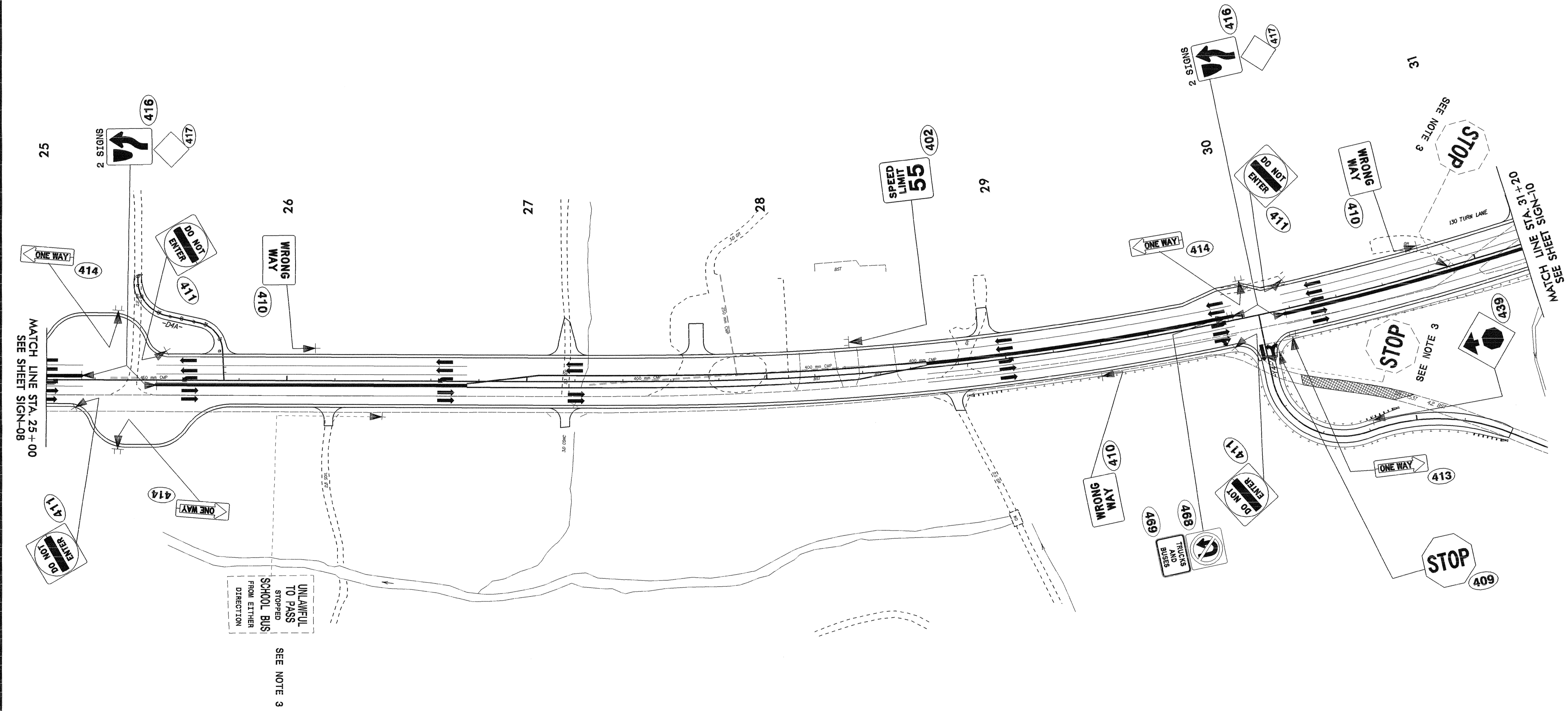
EXISTING AND PROPOSED SIGNS -L- STA. 25+00 TO 31+20 US 19
