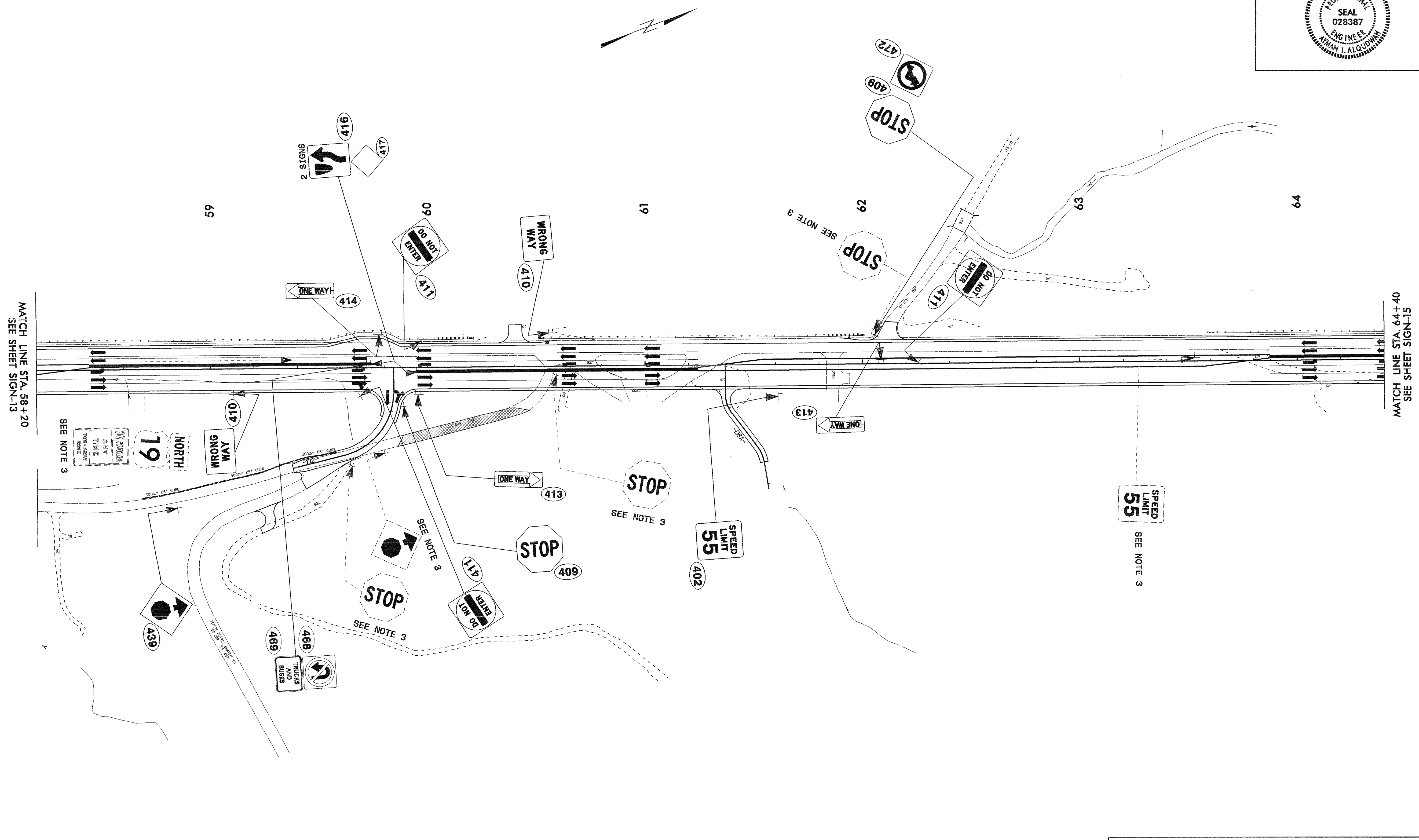
EXISTING AND PROPOSED SIGNS -L- STA. 58+20 TO 64+40 US 19
