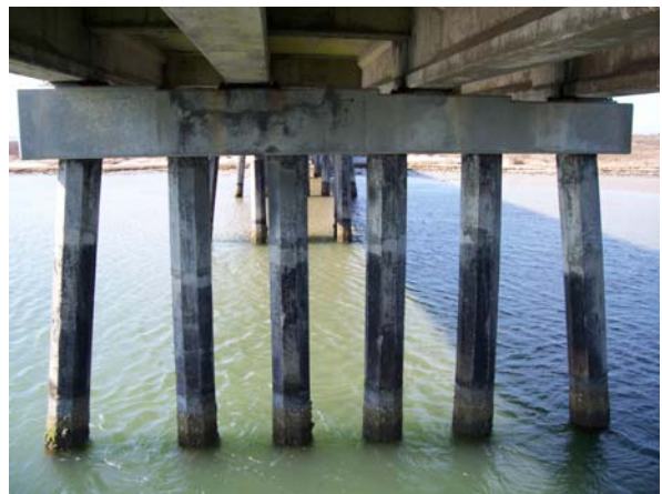
Bent 93, south elev
