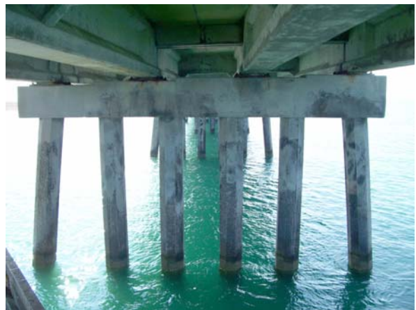
Bent 102: north elevation
