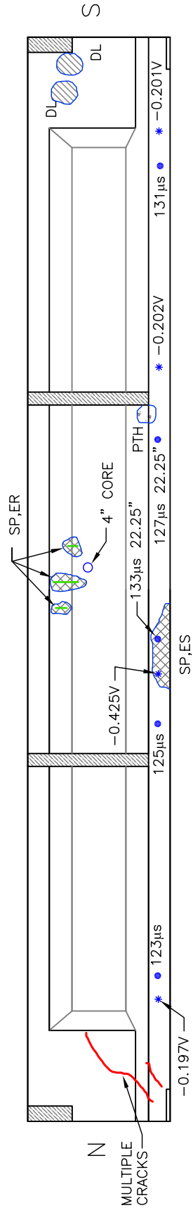
G1—West Elevation
