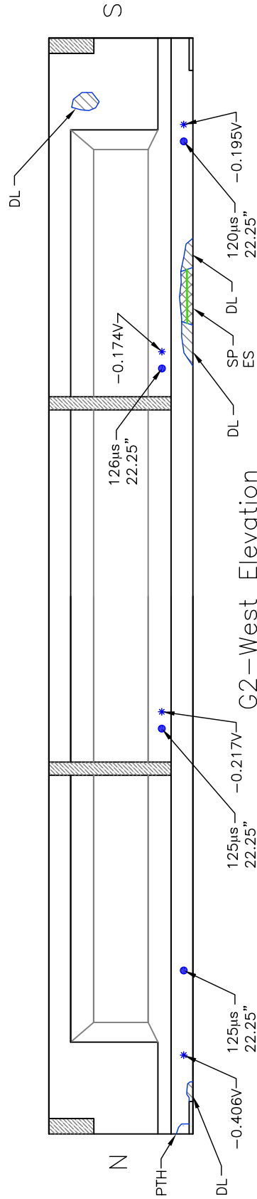
G2--East Elevation
