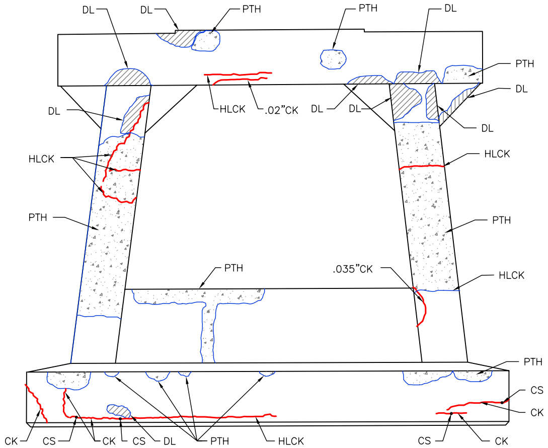
South Elevation
