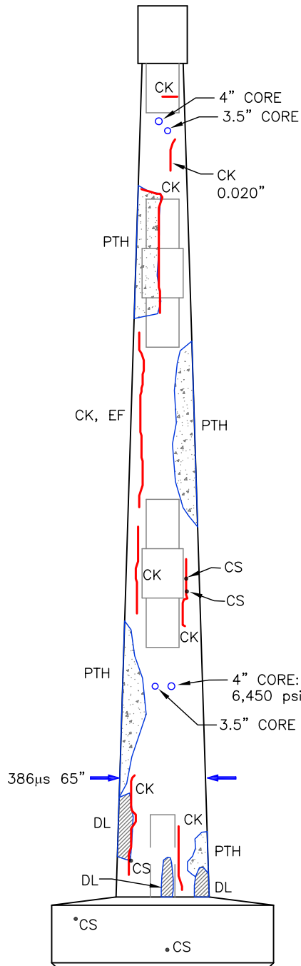
West Ext. Side
