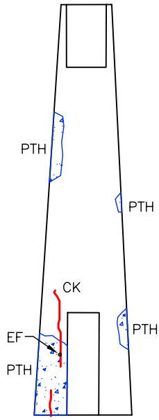
West Int. Side
