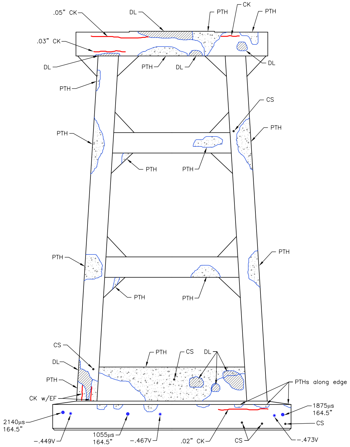
North Elevation
