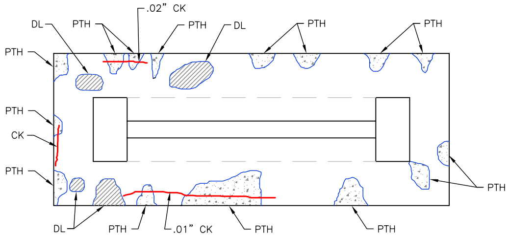
West ← Top of Pile Cap → East
