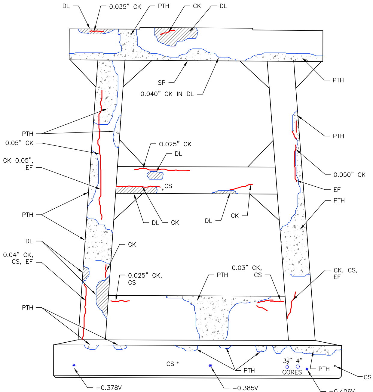
South Elevation
