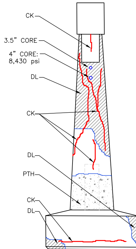
East Ext. Side
