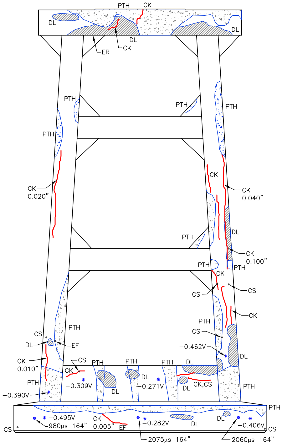
North Elevation
