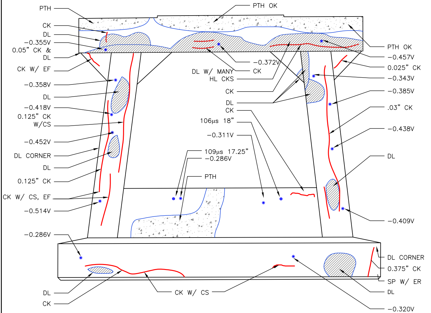
North Elevation
