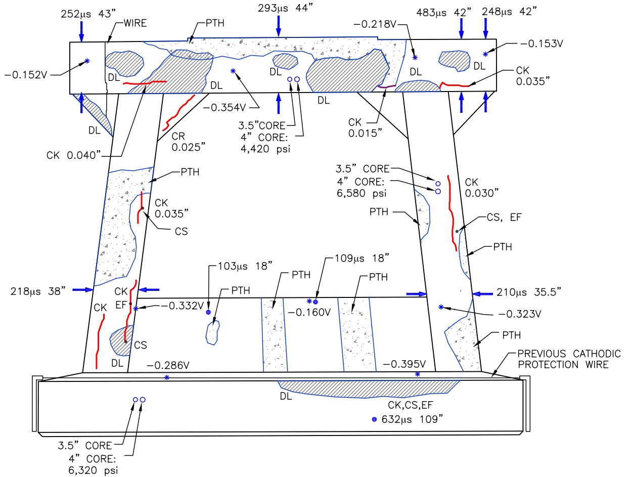
South Elevation
