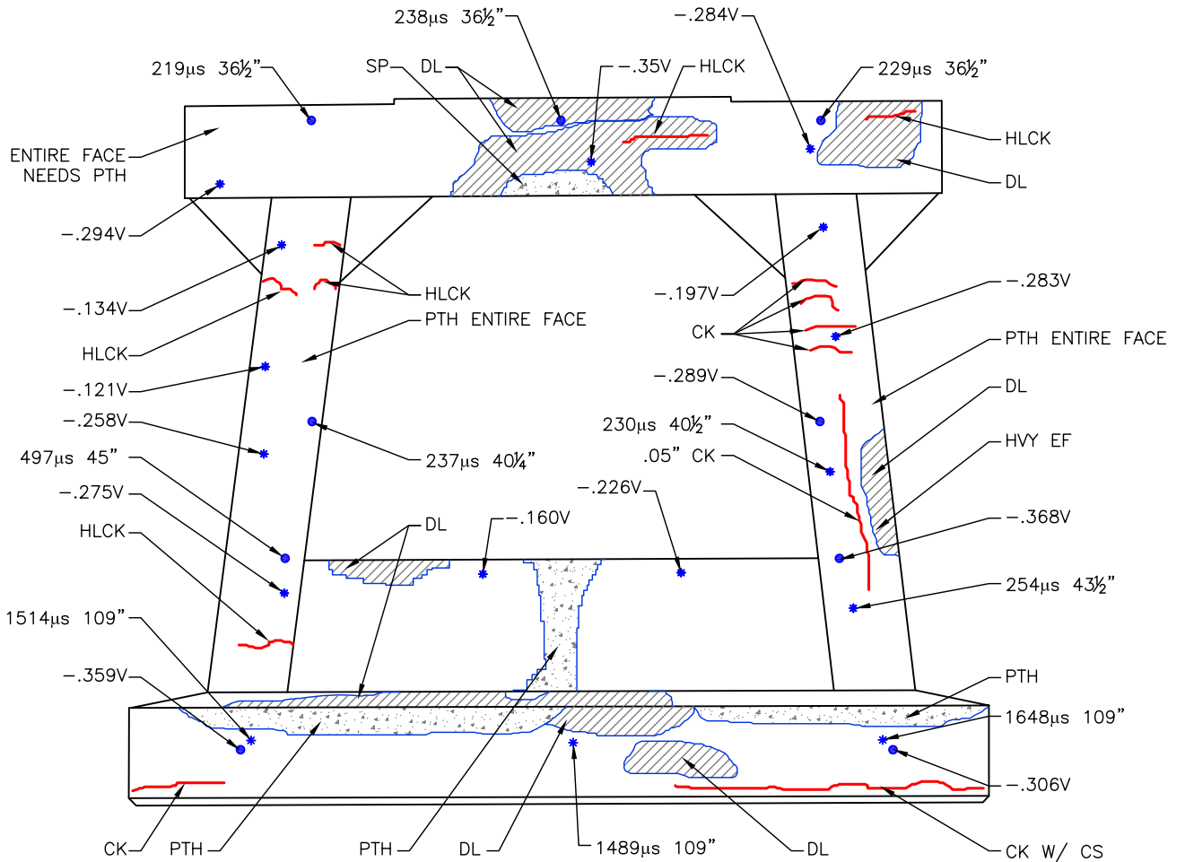
South Elevation
