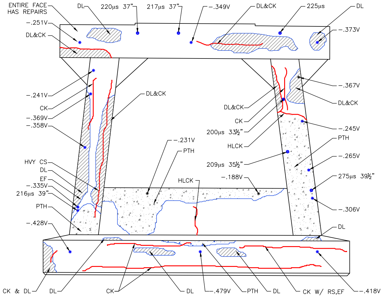
North Elevation
