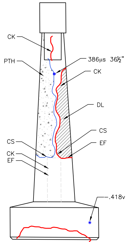
East Ext. Side
