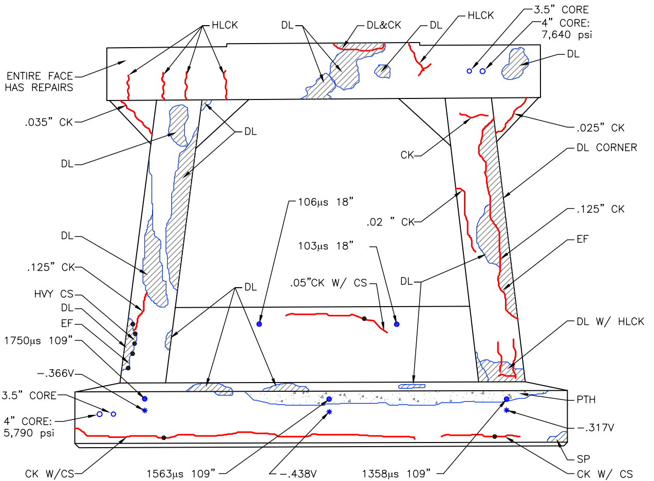
South Elevation
