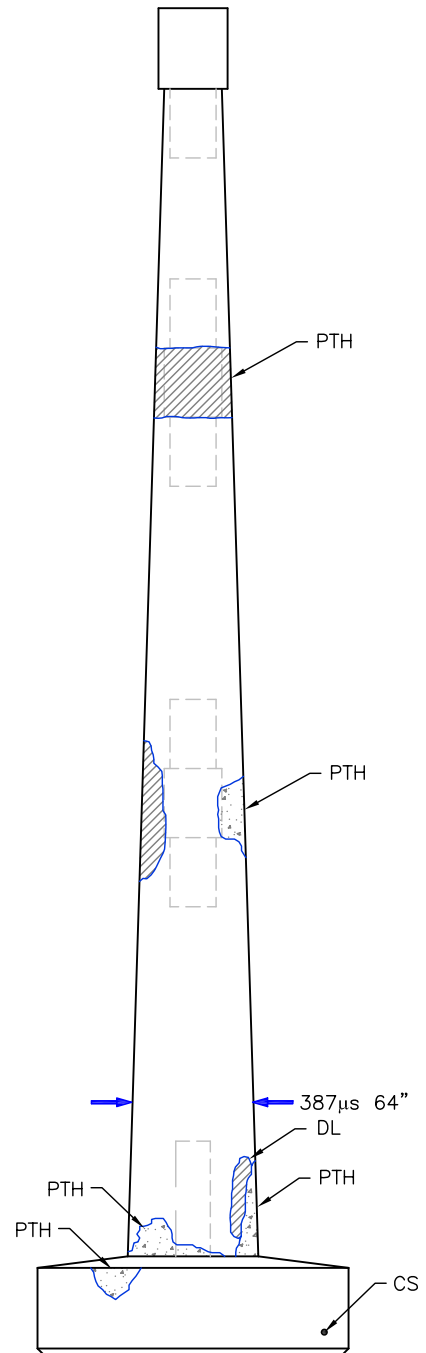
East Ext. Side
