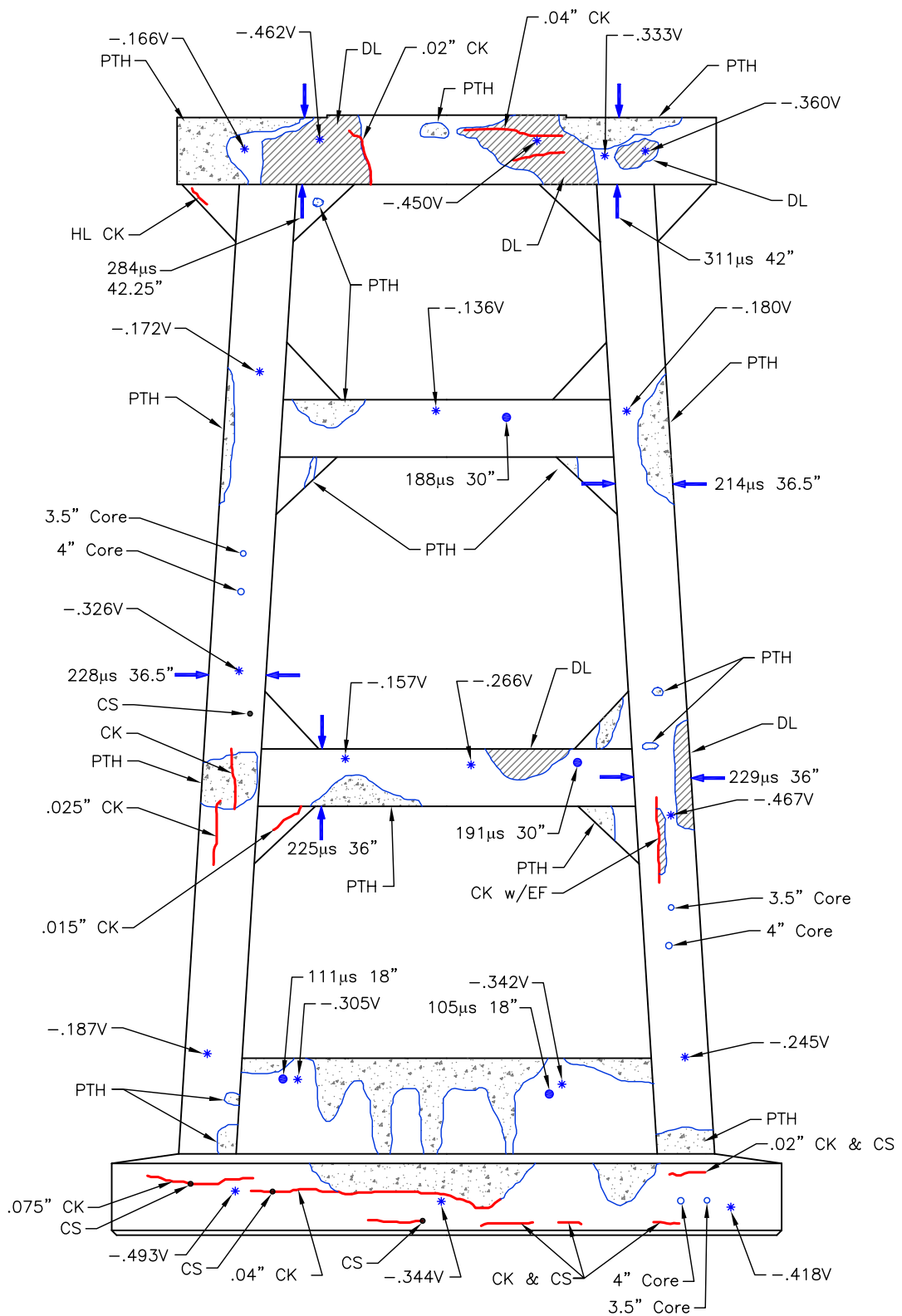
South Elevation
