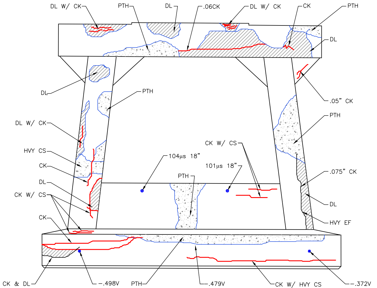
North Elevation
