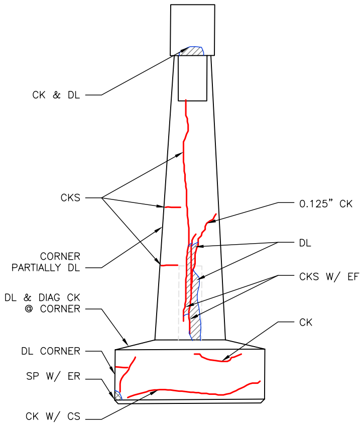
West Ext. Side
