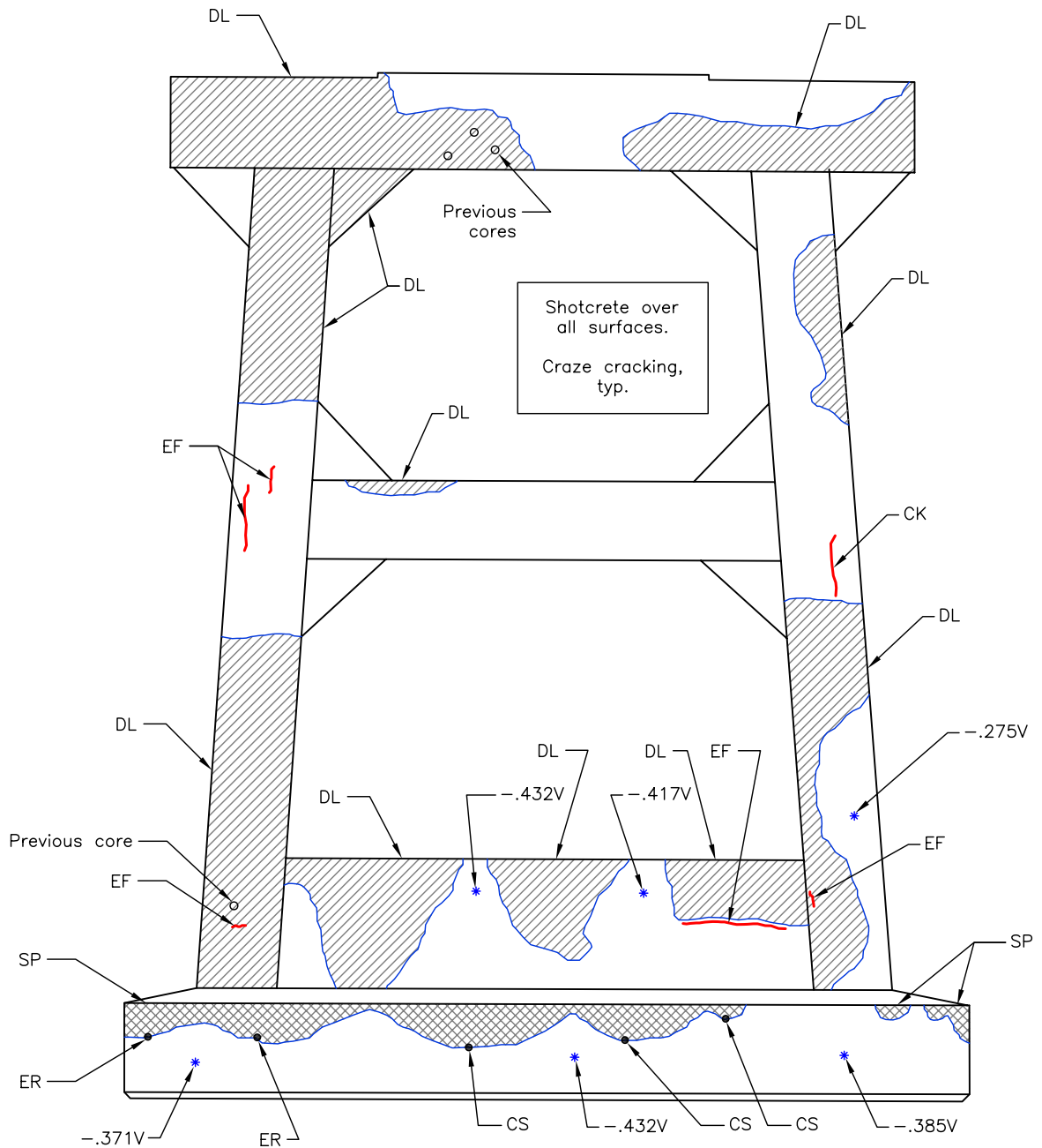
North Elevation
