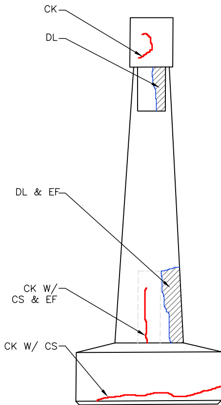
West Ext. Side
