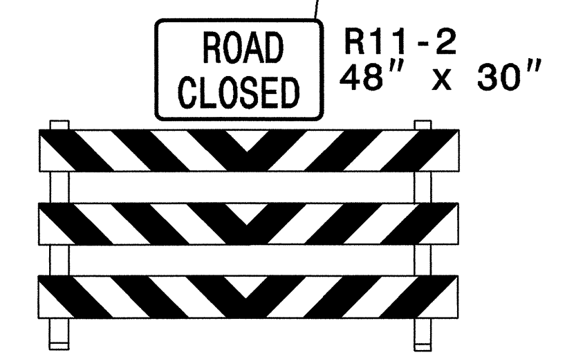
TYPE III BARRICADE SEE NOTE 10, SHEET TCP-18
