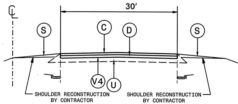
TYPICAL NO. 3 USE FOR MAP 4
