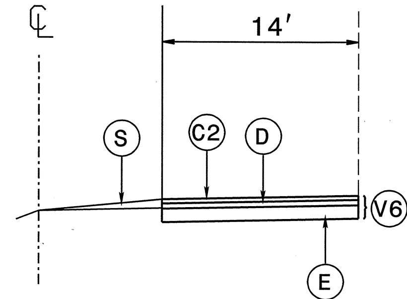
DETAILS OF FULL DEPTH PAVEMENT REPLACEMENT OF ABOUT 320' LONG TURN LANE FROM US-64 ON TO I-440 EASTBOUND
