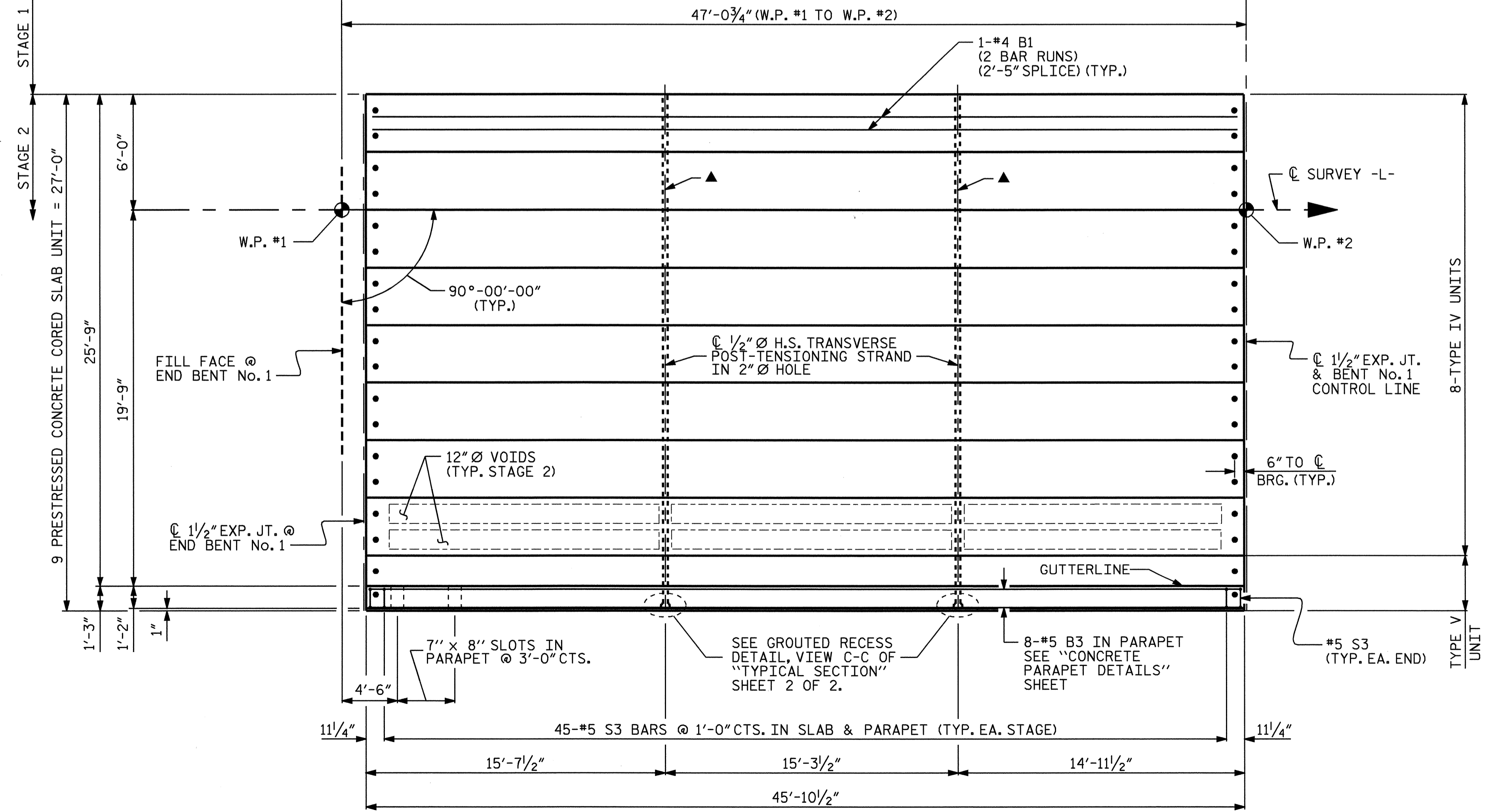
PLAN OF SPAN "A" (STAGE 2)
