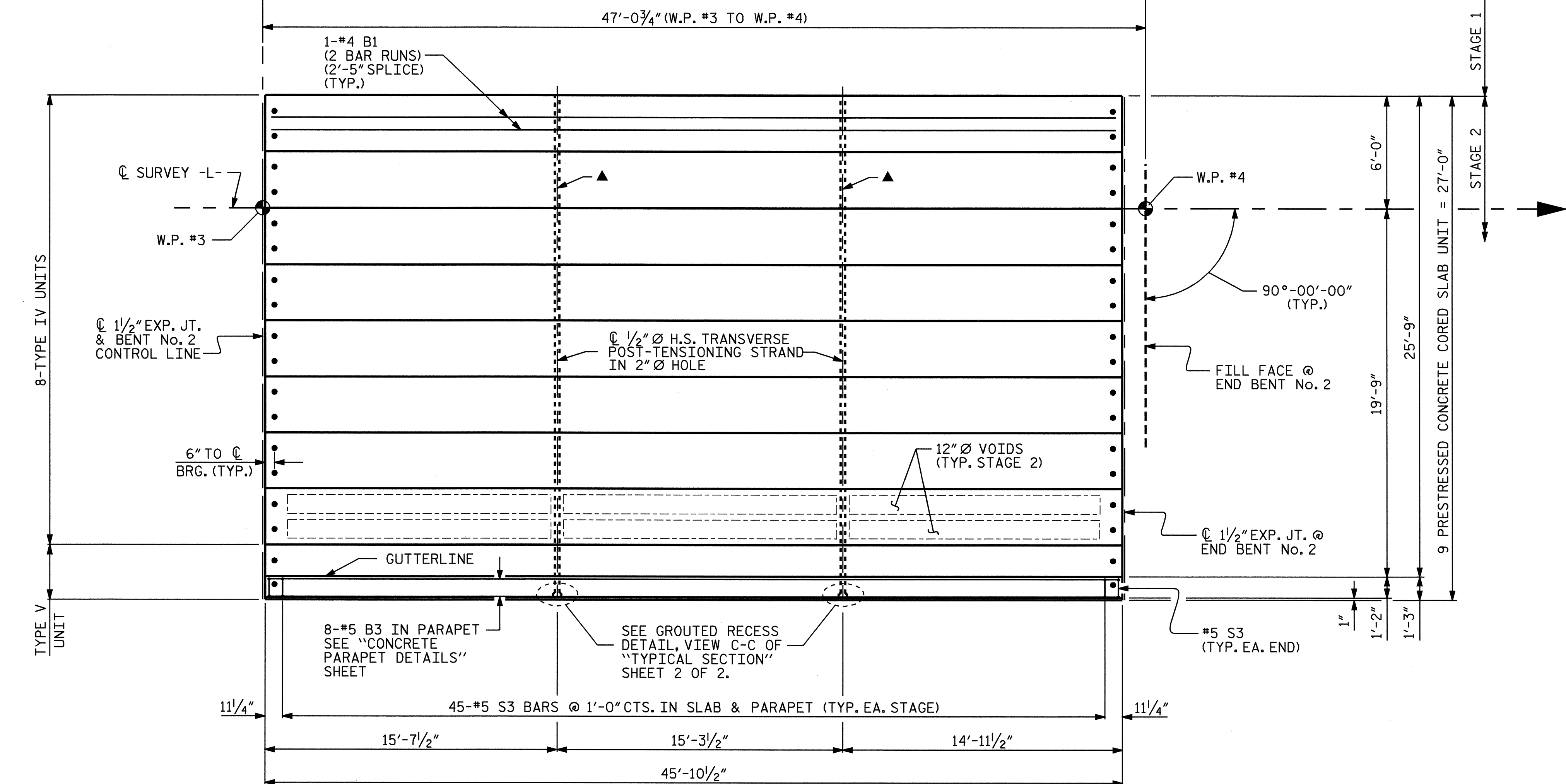
PLAN OF SPAN "C" (STAGE 2)
