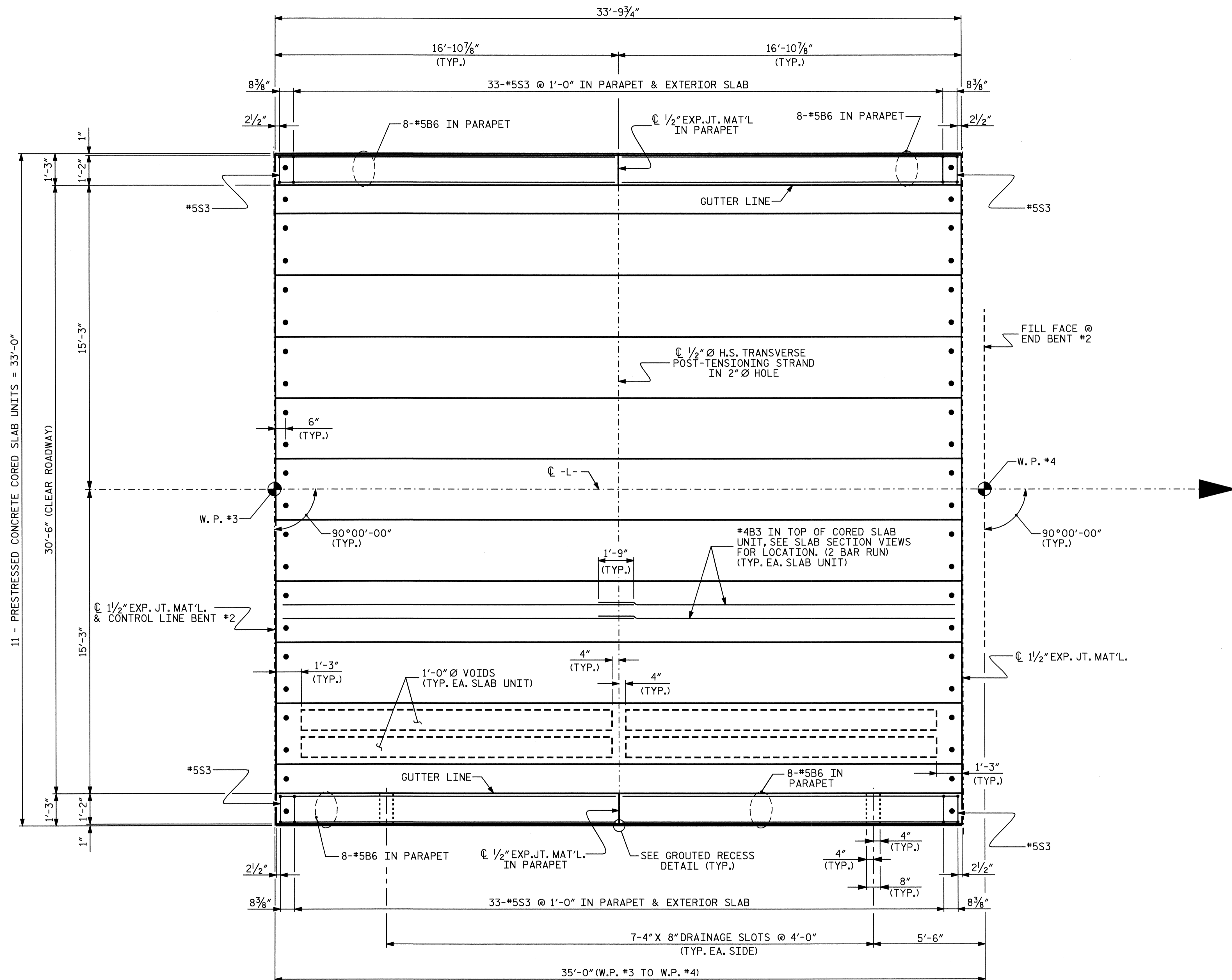
PLAN OF SPAN C
