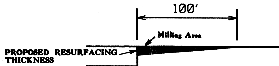
MILLING DETAIL AT BRIDGE APPROACHES
