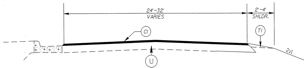
TYPICAL SECTION NO. 9
