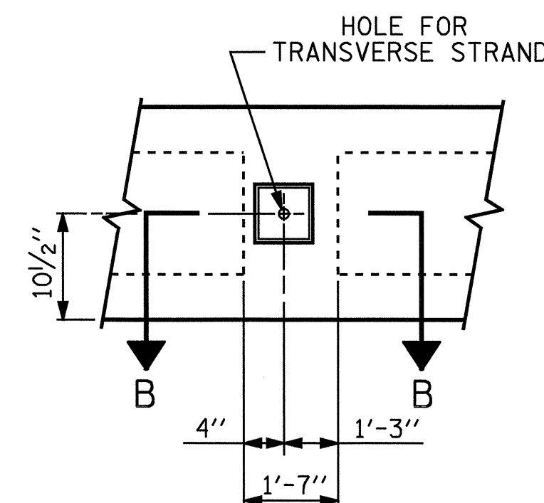
ELEVATION VIEW
