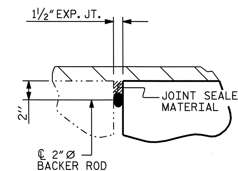
DETAIL A
