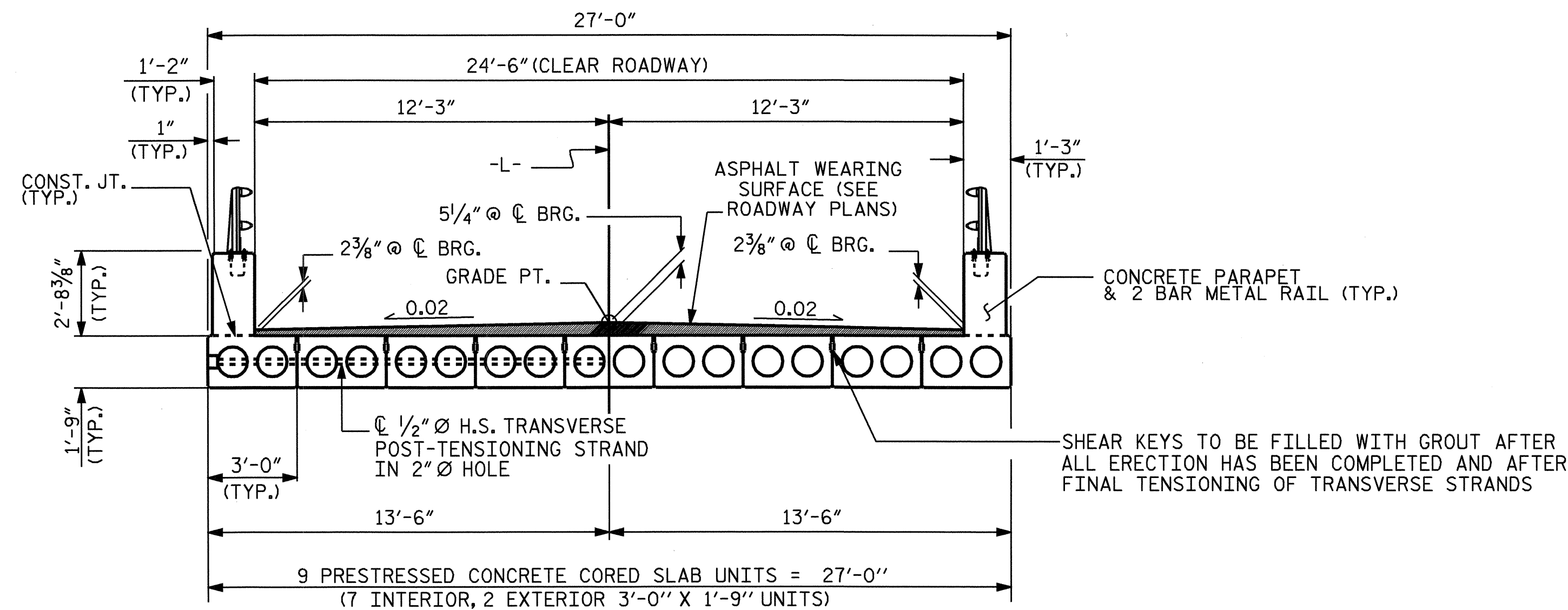
HALF SECTION @ POST-TENSIONING LOCATIONS
