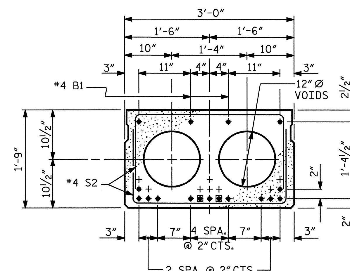
INTERIOR SLAB SECTION
