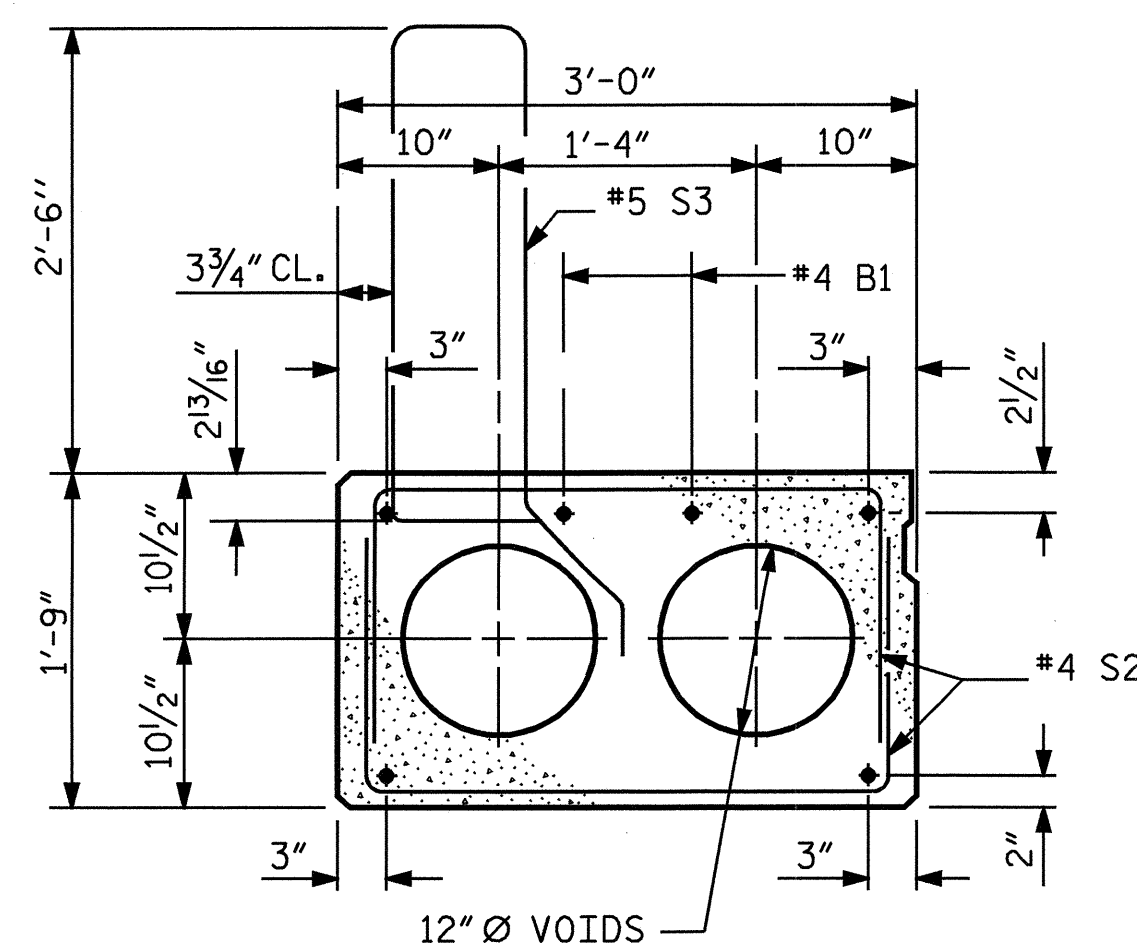
EXTERIOR SLAB SECTION
