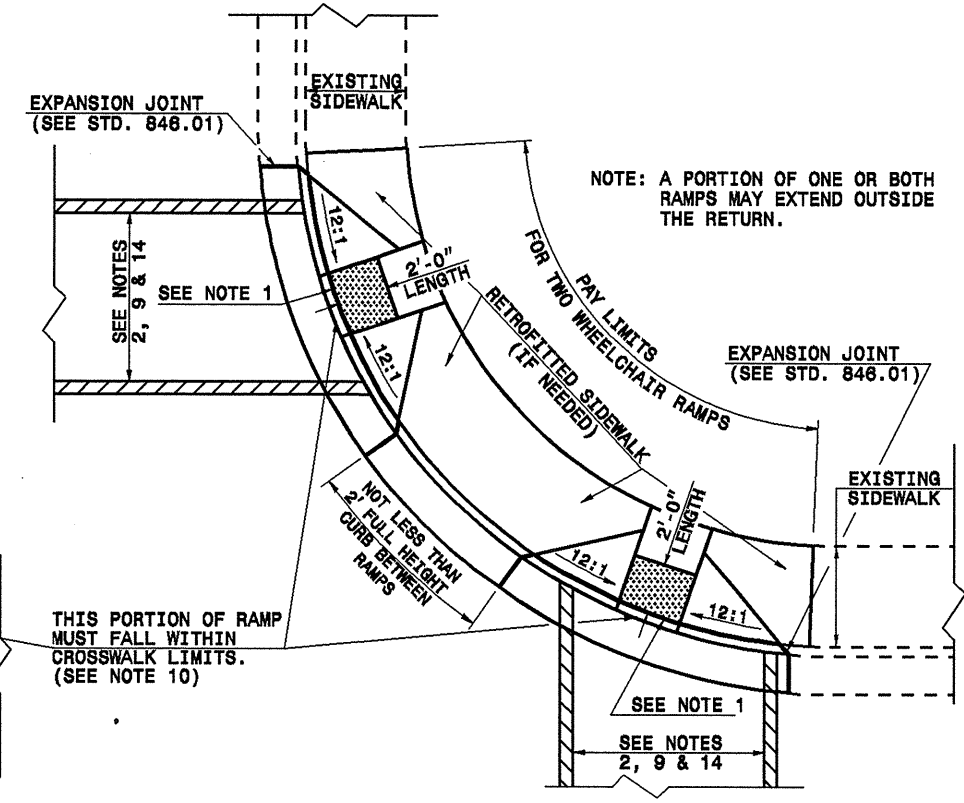
PLAN VIEW
